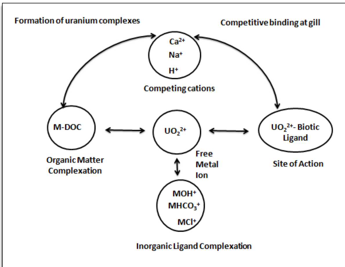
Figure 1. Schematic outline of BLM showing competitive interaction of UO_2^{2+} with other ions in solution and uptake in fish. M represents uranium species (Di Toro et al., 2005).
