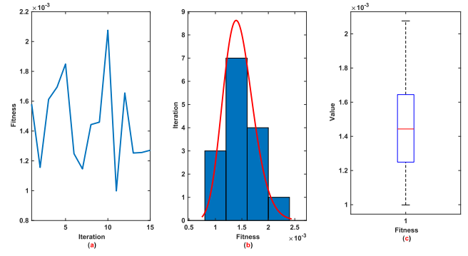
FIGURE 9. Example 1: FIT examination: (a): Trajectory; (b): Histogram; (c): Box plot.
