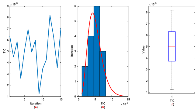
FIGURE 12. Example 2: TIC examination: (a): Trajectory; (b): Histogram; (c): Box plot.
