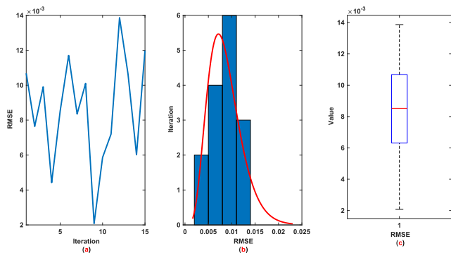
FIGURE 13. Example 2: RMSE examination: (a): Trajectory; (b): Histogram; (c): Box plot.
