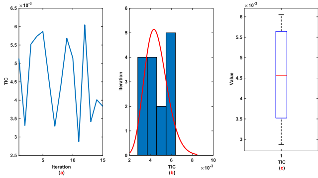
FIGURE 6. Example 1: TIC examination: (a): Trajectory; (b): Histogram; (c): Box plot.
