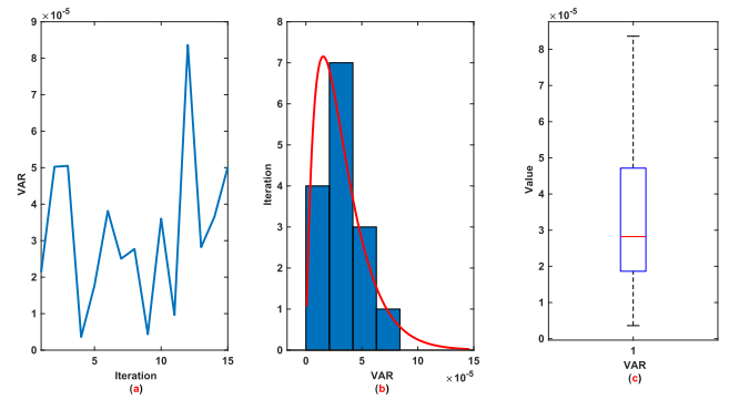
FIGURE 14. Example 2: VAR examination: (a): Trajectory; (b): Histogram; (c): Box plot.
