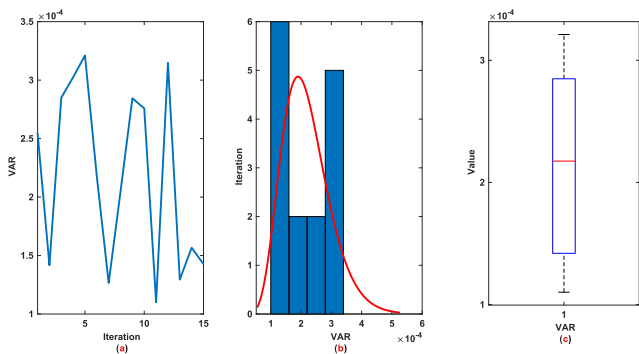
FIGURE 8. Example 1: VAR examination: (a): Trajectory; (b): Histogram; (c): Box plot.
