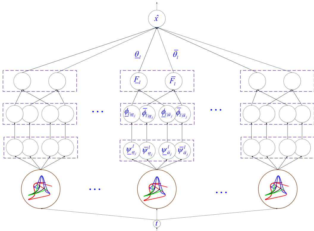
FIGURE 2. A general view of the proposed T3-FLS solution estimator.
