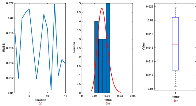
FIGURE 7. Example 1: RMSE examination: (a): Trajectory; (b): Histogram; (c): Box plot.
