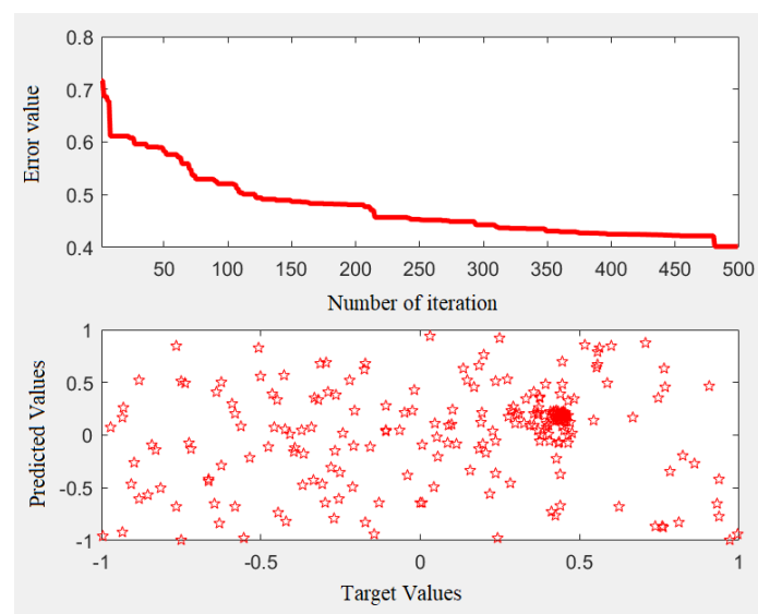
Figure 5. MLP–GA training process.
