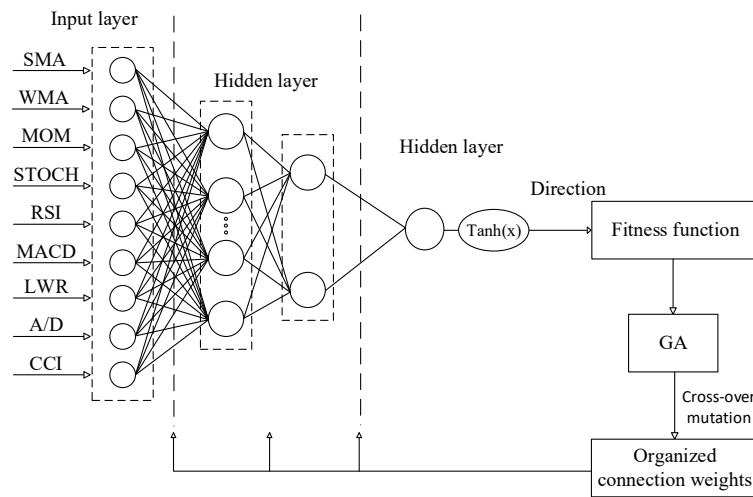
Figure 3. The flowchart of the MLP-GA algorithm.
