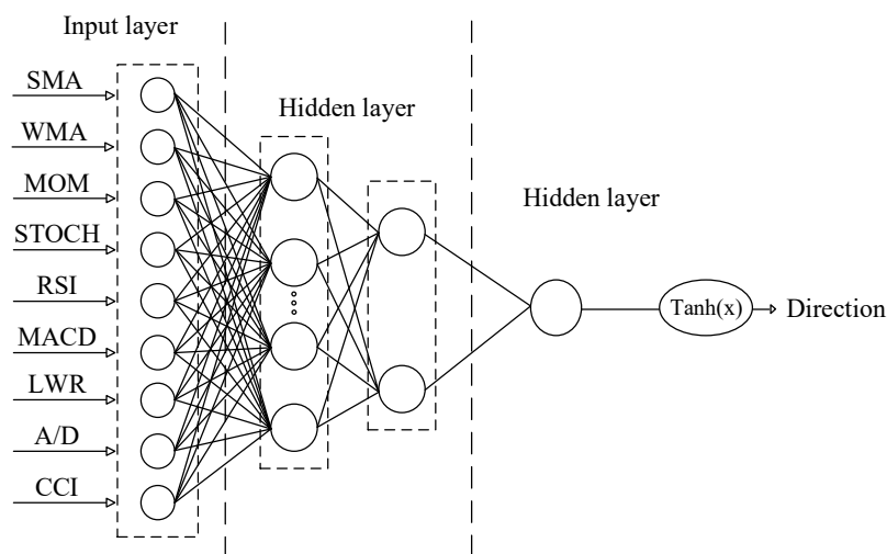
Figure 1. The architecture of MLP.
