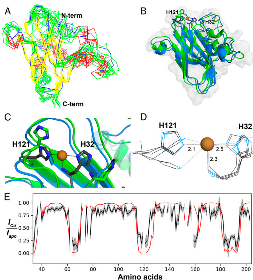
Fig. 1. Structures of apo - and Cu(I)-B/LPMO10A. (A) Ensemble of the 10 lowest-energy conformers of apo -B/LPMO10A (PDB ID code 5LW4) in stereo representation. Helices are colored red, loops are colored green, and strands are colored yellow; the lowest CYANA target energy conformer is colored blue. The overall backbone rmsd of the ensemble is 2.41 Å, while the rmsd of the regions containing \alpha -helices (residues 41–47, 57–61, 82–84, 89–94, and 159–162) and \beta -sheets (residues 33–36, 37–40, 103–107, 110–117, 125–132, 150–154, 164–168, 175–184, 185–190, and 191–201) is 1.48 Å. (B) Overlay of apo -B/LPMO10A (green) and Cu(I)-B/LPMO10A (PDB ID code 6TWE; blue). The copper atom is shown as an orange sphere, and the side chains of His32 and His121 are shown as sticks. The backbone (C α , N, C β ) rmsd between the apo ensemble and the Cu(I) ensemble is 0.9 Å. (C) Zoomed-in view of the overlay in B showing details of the copper site. (D) Ensemble of five lowest-energy conformers of Cu(I)-B/LPMO10A, showing the copper site. Average distances from each N atom to the Cu atom are indicated. (E) PRE effects upon adding Cu(II) to apo -B/LPMO10A. The black line shows the normalized H N , N signal intensity upon addition of Cu(II) to 13 C- and 15 N-labeled apo -B/LPMO10A in a 1:2 ratio, relative to the intensity for the apo -enzyme, with errors shown in gray. The red line shows PREs calculated using the Cu(I)-B/LPMO10A ensemble. Gaps in the data represent missing assignments for amino acid residues (e.g., Pro).
