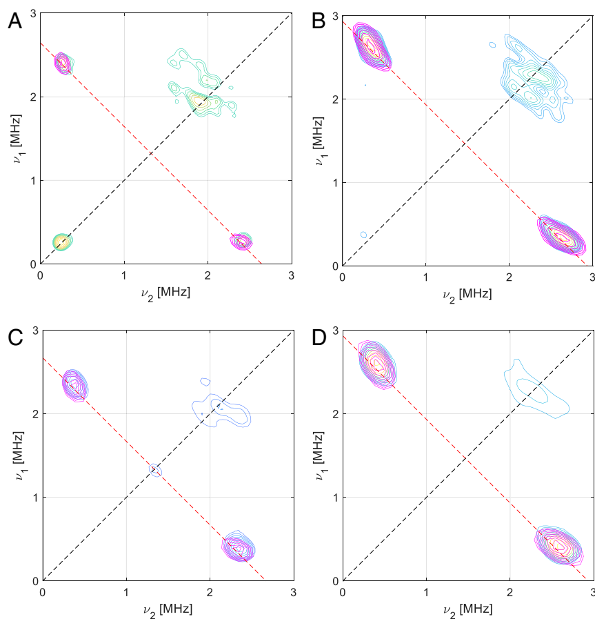
Fig. 4. ^{15}\text{N} -HYSCORE spectra and simulations of ^{63}\text{Cu}\text{-}^{15}\text{N-B/LPMO10A} (A and B) and ^{63}\text{Cu}\text{-}^{15}\text{N-B/LPMO10A} with squid pen \beta -chitin (C and D). Numerical simulations (in pink) were obtained with the values reported in Table 3. (A) ^{63}\text{Cu}\text{-}^{15}\text{N-B/LPMO10A} near g_{\perp} with \tau = 136 ns at 3,395 G; (B) ^{63}\text{Cu}\text{-}^{15}\text{N-B/LPMO10A} near g_{\parallel} with \tau = 136 ns at 3,060 G; (C) ^{63}\text{Cu}\text{-}^{15}\text{N-B/LPMO10A} with squid pen \beta -chitin near g_{\perp} with \tau = 200 ns at 3,390 G; (D) ^{63}\text{Cu}\text{-}^{15}\text{N-B/LPMO10A} near g_{\parallel} with \tau = 200 ns at 3,090 G.
