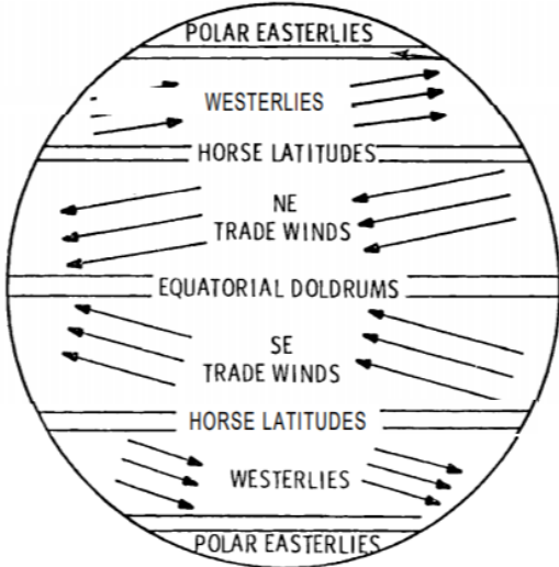
Figure 1 – Surface winds of the general circulation (Hiester & Pennell, 1981)
