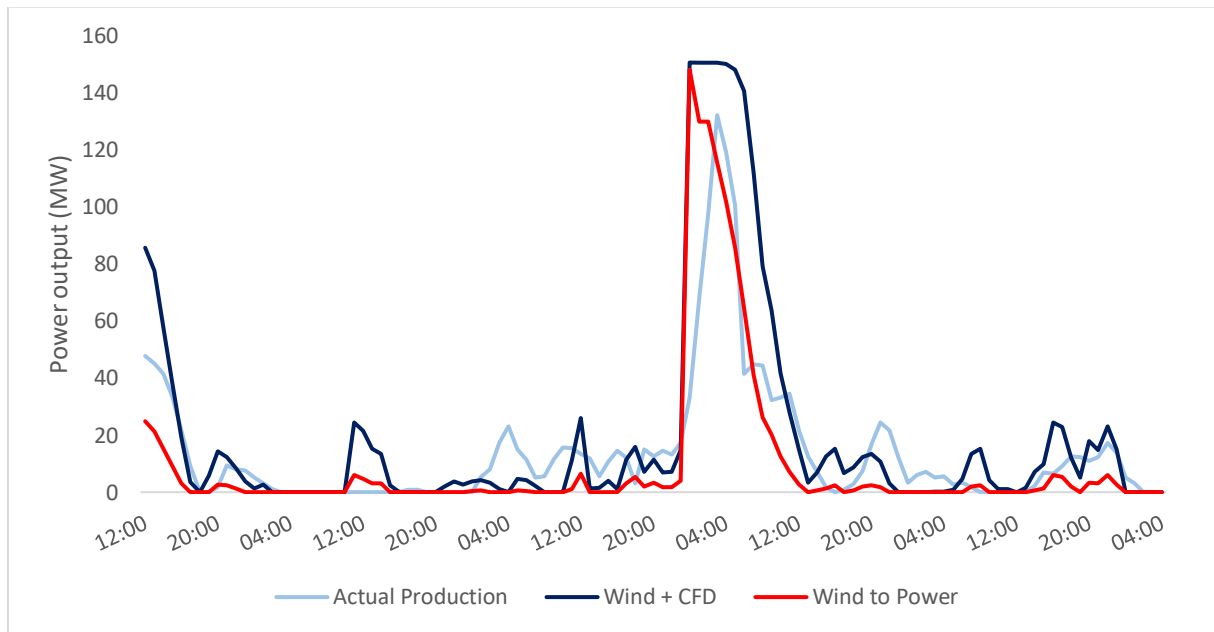
Figure 31 – Rapid change in wind speed at Smøla wind farm
