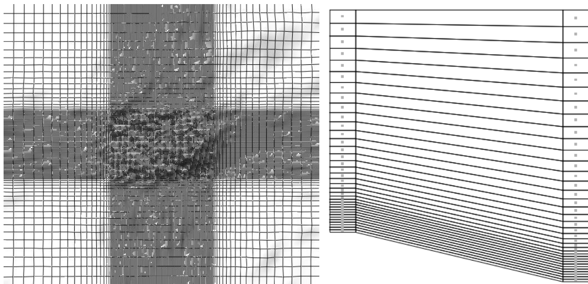
Horizontal grid resolution (left) and schematic view of the vertical grid resolution (right)
