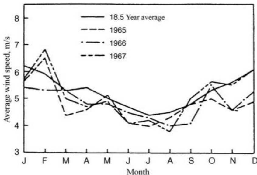
Figure 3 – Seasonal changes in wind speeds (Hiester & Pennell, 1981)
