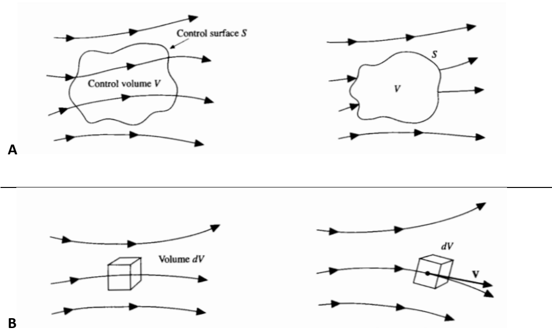
Figure 8 – A) The finite volume method. B) Infinitesimal fluid element (Anderson & Wendt, 1995)
