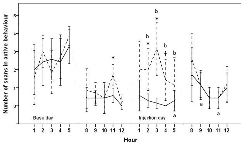
Fig. 3. The average number of scans ( \pm 2 SE) in active behaviors on BASE day (left) and the day of LPS injection (INJ, right). The dashed line represents SAL and the uninterrupted line LPS pigs. Hours are given in relation to the time of LPS injection. Treatment effects (LPS vs SAL) are denoted with * ( p < .05 ) and † ( p < .1 ) and day effects (BASE as compared to INJ within treatment) with a ( p < .05 ) for LPS and b ( p < .05 ) for SAL.
