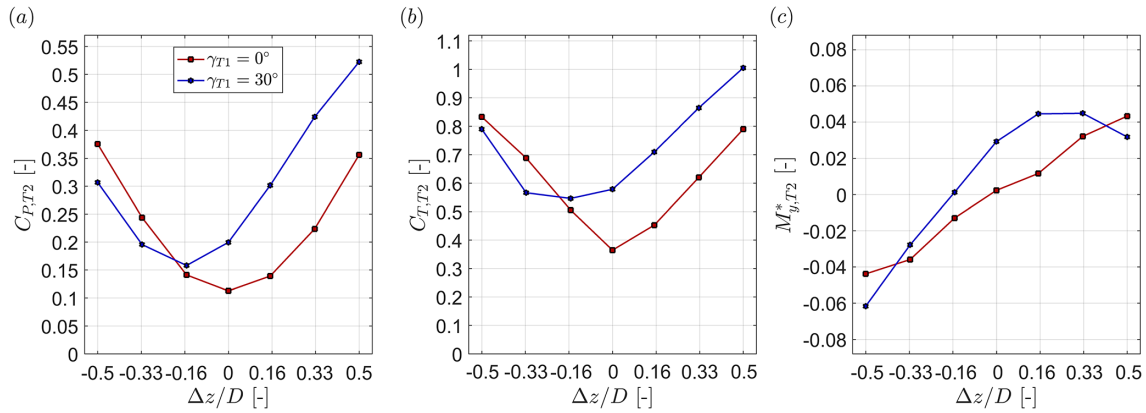
Figure 8. Downstream turbine (a) power coefficient, (b) thrust coefficient and (c) normalized yaw moment as a function of its lateral offset position \Delta z/D . The downstream turbine yaw angle is kept constant at \gamma_{T2} = 0^\circ . The downstream turbine T2 is located at x/D = 3 . The turbines are exposed to inflow B.
