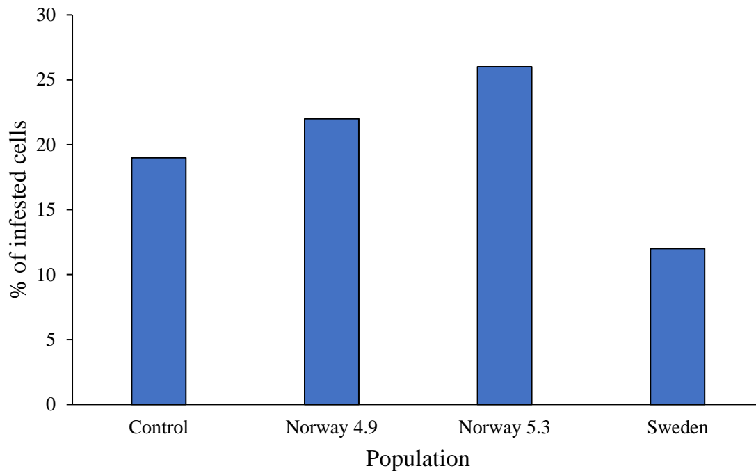
Figure 5: The proportion of honey bee brood cells that were infested with varroa mites and recapped in each population. Number of artificially infested cells in each population: Control N= 271, Norway 4.9 (small cell comb) N= 270, Norway 5.3 (standard cell comb) N= 162, Sweden N= 317.
