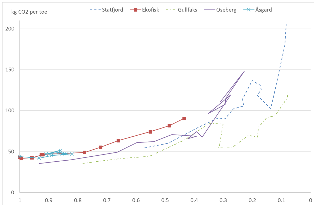
Figure A1. Relationship between annual production level (as a share of peak production) and emission intensity for the five biggest non-electrified Norwegian fields*
