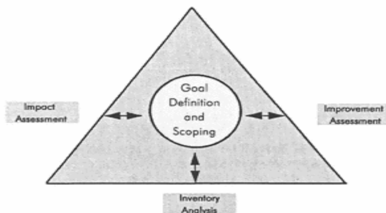
Figure 2-5: SETAC Triangle.
