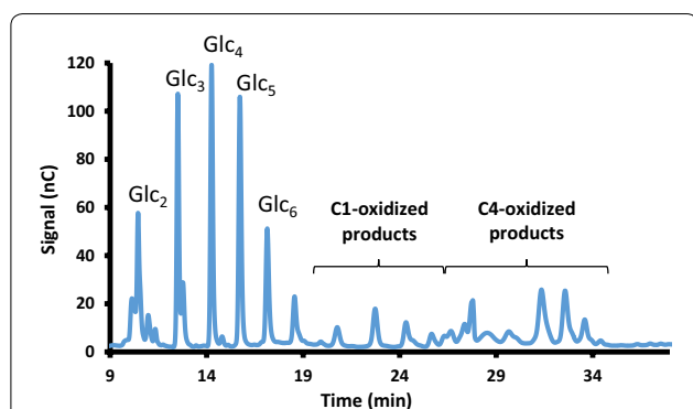
Fig. 3 HPAEC chromatogram showing the soluble products obtained after degradation of PASC by TaLPMO9A . The profile indicates a dominating C4-oxidizing activity with minor C1-oxidizing activity
