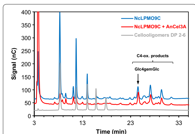
Fig. 2 HPAEC chromatogram showing the effect of AnCel3A \beta -glucosidase on the reaction products of NcLPMO9C , a C4-oxidizing LPMO. The blue curve shows products (Glc 2 , Glc 3 , Glc 4 , and oxidized sugars) generated from PASC by NcLPMO9C . The red curve shows the product profile after AnCel3A has been added to the NcLPMO9C product mix. The grey curve shows celoo-oligosaccharide standards from Glc 2 to Glc 6 , eluting according to length, with Glc 2 elution first. It is clearly seen that treatment with AnCel3A leads to production of Glc ( red peak to the left) and consumption of the native celoo-oligosaccharides. However, the C4-oxidized products were not degraded by AnCel3A
