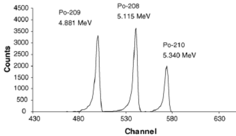
Figure 12: Graphic representation of alpha spectrum depicting energies of different polonium isotopes (Vesterbacka & Ikaheimonen, 2005)
