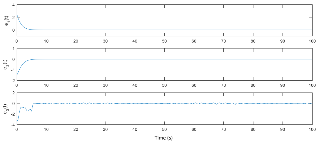
Figure 5. Synchronization error dynamics of unknown time-delay Jerk master slave chaotic systems (25), (26) using the proposed robust adaptive control strategy where it is activated at t = 5 s.
