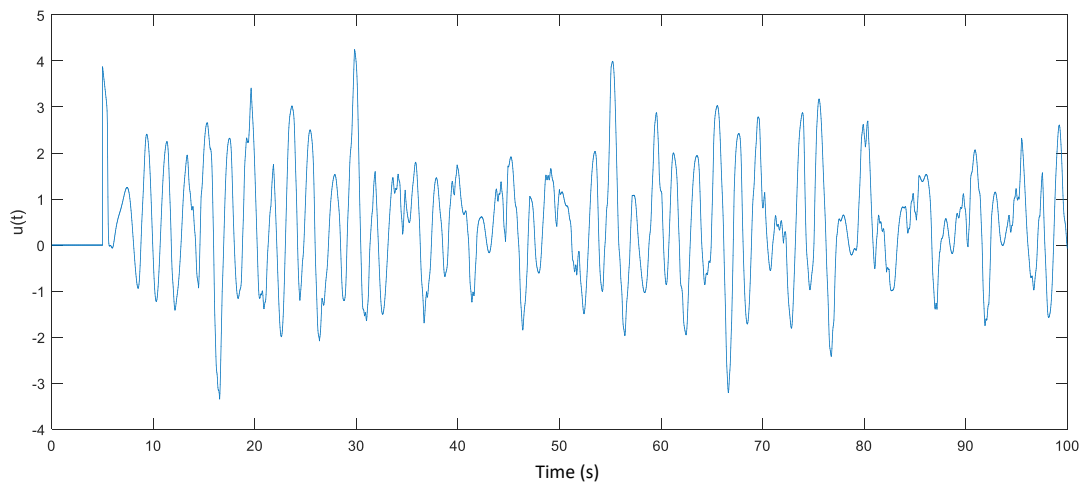
Figure 6. Control signal based on the proposed robust adaptive control strategy (11) where it is activated at t = 5 s.
