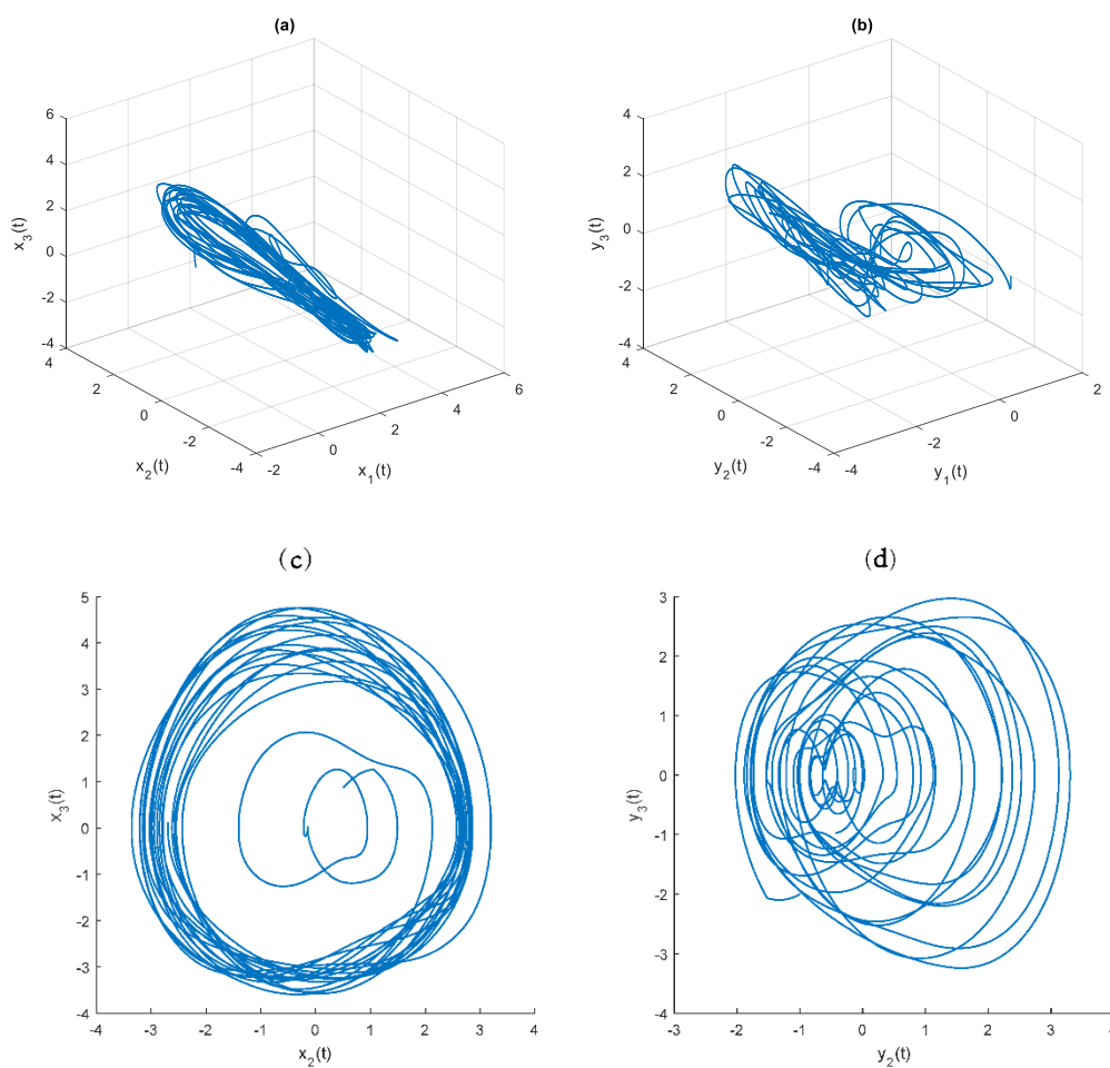
Figure 1. Exhibits chaotic behaviors of the fractional-order modified Jerk system without the controller. (a) The phase portrait of the master system (25), (b) the phase portrait of the slave system (26), (c) the plan x_2 - x_3 of master system, and (d) the plan y_2 - y_3 of the slave system.
