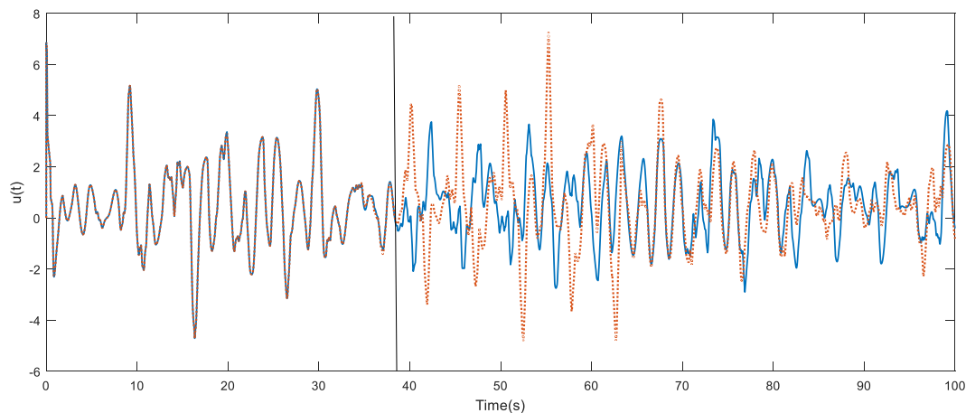
Figure 9. Controller signals based on the proposed robust adaptive control strategy (11) where it is activated at t = 5 s. The solid line is the control signal based on the fixed unknown time delays \tau_1 = 0.45 , \tau_2 = 0.1 and the dotted line is the control signal based on step-change of unknown variable time delays \tau_1 = 0.45 to \tau_1 = 0.5 at t = 38.45 s and \tau_2 = 0.1 to \tau_2 = 0.7 at t = 38.45 s.
