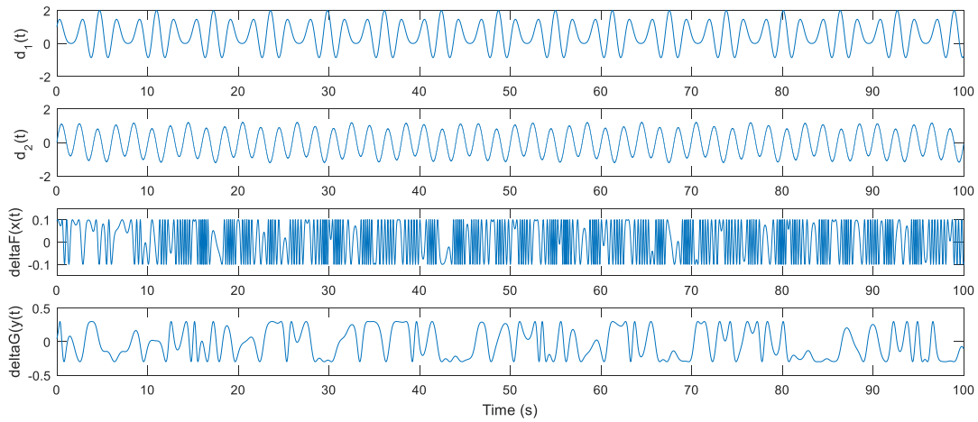
Figure 3. Disturbances ( d_1(t) , d_2(t) ) and uncertainties ( \Delta f(x(t), t) , \Delta g(y(t), t) ) in the master and slave systems (25), (26).
