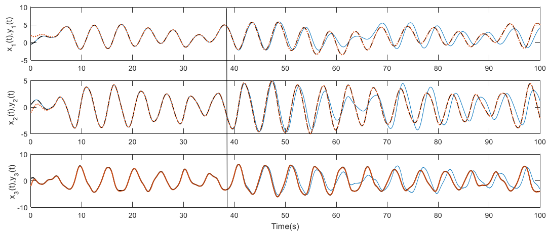
Figure 8. The robust synchronization presses of systems (25), (26) with unknown variable time delays based on the proposed adaptive control strategy where it is activated at t = 5 s. Solid lines are the dynamics of the master system for \tau_1 = 0.45 , dashed-dotted lines are the dynamics of the master system based on step-change \tau_1 = 0.45 to \tau_1 = 0.5 at t = 38.45 s, and dotted lines are the dynamics of the slave system based on step-change \tau_2 = 0.1 to \tau_2 = 0.7 at t = 38.45 s.
