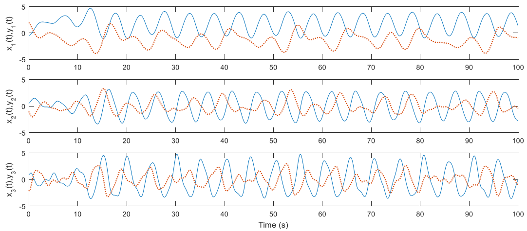
Figure 2. Representation of the dynamics of the master and slave systems (25), (26) without the controller. Solid lines are the dynamics of the master system and dotted lines are the dynamics of the slave system.
