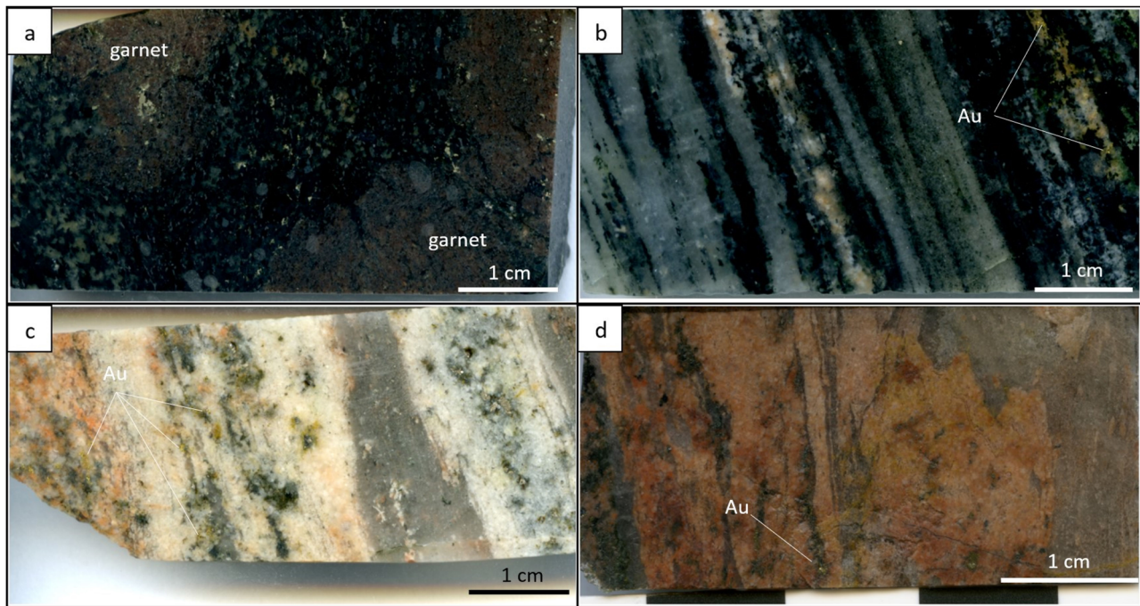
Figure 3. Images of samples selected for mineral geochemistry and P - T work including: (a) garnet-bearing amphibolite at ~800 m north of Tick Hill pit (sample TH99); (b) gold-bearing, amphibole-rich calc-silicate (sample TH46); and (c, d) quartz-feldspar mylonite (samples TH55, THM22, respectively).
