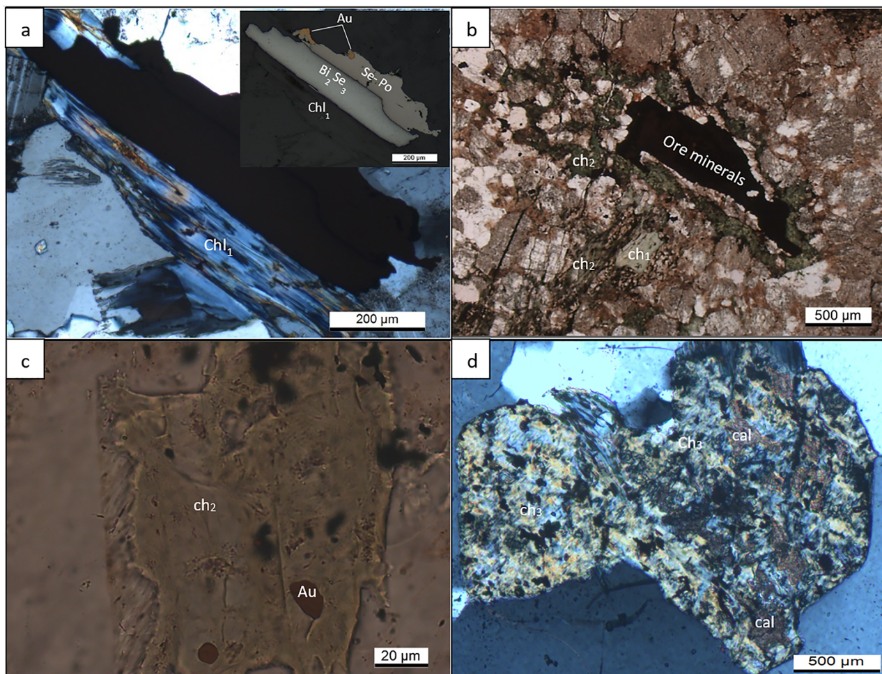
Figure 6. Photomicrographs showing D_3 alteration minerals in various quartz–feldspar mylonite units in the most strongly altered core of the ore zone. (a) Early D_3 chlorite, ( ch_1 ) with morphology of initial mineral of biotite (Le et al. , 2021a) and associated with bismuth selenide ( Bi_2Se_3 ), selenide-rich pyrothite (Se–Po) and gold (sample TH55), with an inserted image captured from reflected light. (b) Chlorite 2 ( ch_2 ) replacing chlorite 1 ( ch_1 , Le et al. , 2021a) and occurring around an ore mineral (pyrite–chalcopyrite intergrowth) as a reaction rim (sample THM22). (c) Chlorite 2 ( ch_2 ) hosting inclusions of gold (sample TH55). (d) Chlorite 3 ( ch_3 ) intergrown with calcite (cal; sample TH55).
