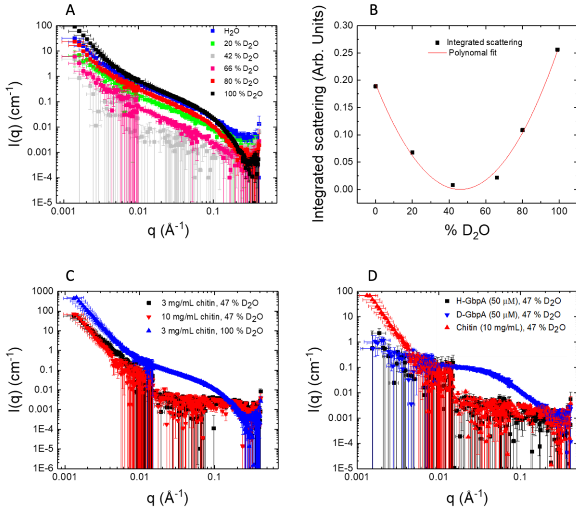
Figure 2 Matching out chitin in SANS experiments A 10 mg/mL chitin was subjected to SANS at six different ratios of \text{D}_2\text{O} to \text{H}_2\text{O} , and the data were plotted as intensities ( I(q) ) vs. the scattering vector ( q ) on double-logarithmic scale. B The scattering for each of the six conditions was integrated, plotted and fitted with a polynomial function, to find the chitin match point at minimal scattering intensity (determined to be at 47% \text{D}_2\text{O} ). C The scattering of chitin in 47% \text{D}_2\text{O} is significantly weaker than in 100% \text{D}_2\text{O} , and is matched out in the middle to high q -range. However, at low- q , chitin could not be perfectly matched out. D In 47% \text{D}_2\text{O} , D-GbpA scatters well in the middle to high q -range, where both chitin and H-GbpA are well matched-out. Error bars represent one standard deviation.
