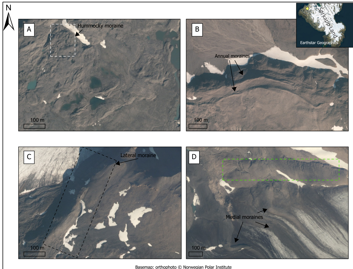
Figure 15: Landforms on the foreland of Gåsbreen. A: Kettle holes and hummocky moraine (white box). B: Annual moraines on the terminal moraine. C: The southern lateral moraine. D: Medial moraines at the end of the glacier. The green box indicates an ice-cored annual moraine.
