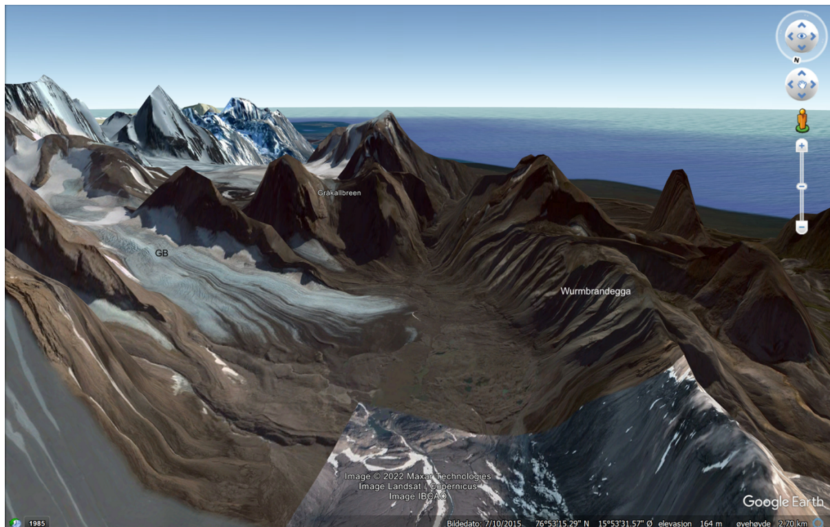
Figure 16: Imagery of the foreland of Gåsbeen (GB) from Google Earth Pro from October 2015. The medial moraines and debris cover on the glacier are clearly seen by the glacier front. Note that north is in the left-bottom of the image and the older imagery in the bottom of the imagery. Exaggeration level: 3.
