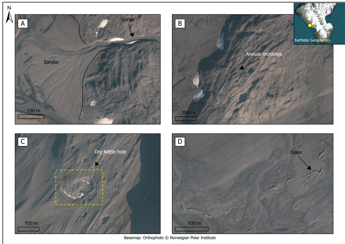
Figure 29: Landforms in and outside of the foreland of Vitkovskjibreen. A: Gorge (black arrow) in the terminal moraine where a sandur has developed outside of the terminal moraine (within black lines). B: Annual moraines (black arrow) on the terminal moraine. C: Dry kettle hole on the eastern lateral moraine. D: A long sinuous esker (black arrow) between the two areas of fluted moraine. Note the break in the esker cut by meltwater.
