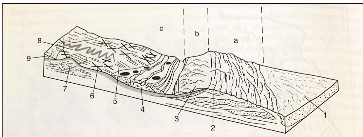
Figure 35: Landsystem model for the margin of a surging glacier from Chapter 11 in Evans (2005). a: outer zone with proglacially sediments that may develop into push moraines on areas with thin sediment cover, b: zone with hummocky moraines on the proximal-glacier side of topographic depressions, c: zone where flutes, CSRs and concertina eskers are present (Evans, 2005). 1: proglacial outwash plain, 2: thrust-block moraine, 3: hummocky moraine, 4: dead-ice covered by pitted and channeled outwash, 5: flutes, 6: CSRs, 7: overridden and fluted thrust-block moraine, 8: concertina esker, 9: glacier with CSRs emerging beneath the glacier (Evans, 2005).
