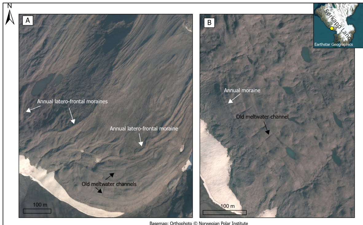
Figure 27: Landforms in the terminal moraine complex of Vitkovskjibreen. A: Examples of annual latero-frontal moraines (white arrows) and old meltwater channels (black arrows) on the eastern lateral moraine. B: Examples of annual moraines (white arrow) and old meltwater channels (black arrow) on the terminal moraine.
