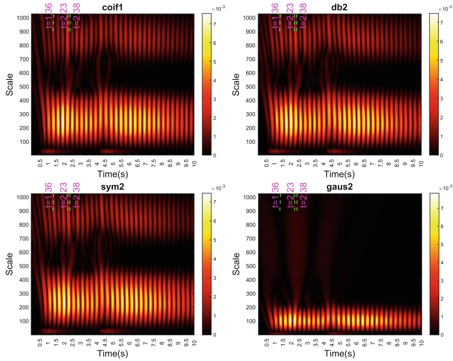
Fig. 7. The absolute coefficient difference of CWT between damaged and undamaged acceleration signal at node 13
