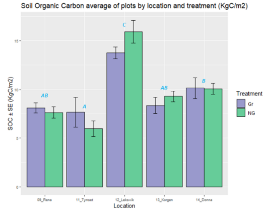
Figure 32: Average SOC stock [kgC/m 2 ] ± standard error (SE) of whole profile classified by treatment and location. Grazed (Gr) sites display as a blue colour, non-grazed (NG) sites as green. Both sites stacked besides each other to their location belongings. Number of samples for every bar; n=5. In addition, uppercase italic blue letters indicate a significant difference between locations independent of site (Gr/NG) ( A, B, AB ). Different letters indicate differences at a level of significance p < 0.05 .
