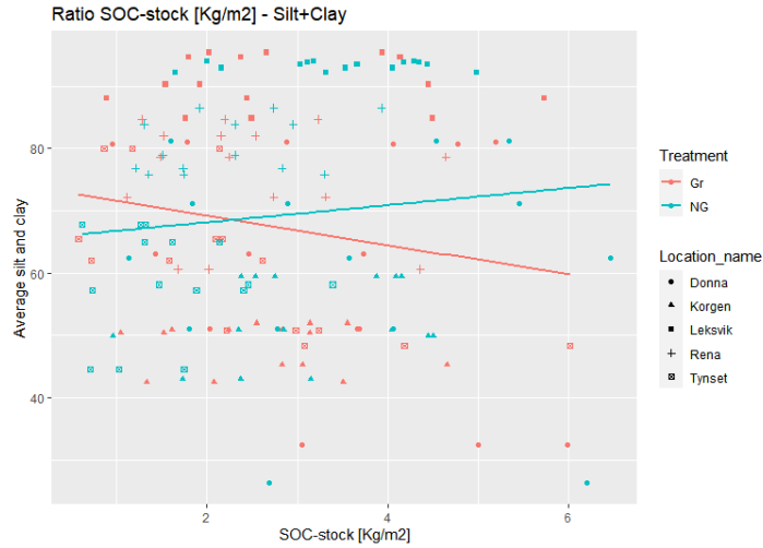
Figure 45: Linear relationship between the average silt and clay fraction and average SOC stock [kgC/m2]. The red line represents the grazed (Gr) sites and the blue the non-grazed (NG) sites. The symbols represent the locations. The organic layer of the profile is not included.
