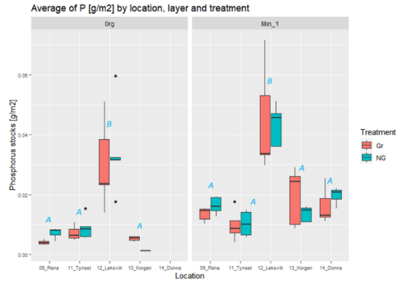
Figure 41: Average P-stocks of layer by treatment and location. The locations are grouped, the name is found on the x axis. The layers are grouped under frame found on top, respectively organic layer and min_1 (0-10 cm) The colour on boxes determine the treatment, grazed (red) and non-grazed (blue). Number of samples in each category displayed in the figure, see appendix 1.6. Notice that location Dønna do not contain a organic layer, and that Korgen, non-grazed site only contain one sample. The boxplots display the maximum and minimum by fully drawn line and outliers is shown with a dot. Horizontal line inside the boxes represents the median of the category. In addition, uppercase italic blue letters indicate a significant difference between locations within each layer (A, B, AB). Different letters indicate differences at a level of significance p<0.05 .
