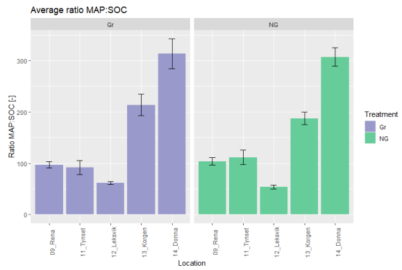
Appendix 13.2: Ratio of mean annual precipitation (MAP) and average SOC stock [kgC/m2] by treatment and location. For treatment grazed (Gr) blue bars and non-grazed (NG) green bars. The locations are given on the x-axis.
