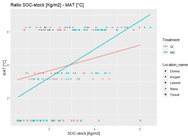
Figure 46: Linear relationship between the MAT [°C] and average SOC stock [kgC/m2] divided by treatment. The red line represents the grazed (Gr) sites and the blue the non-grazed (NG) sites. The symbols represent the locations.
