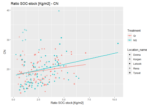
Figure 44: Linear relationship between the average CN and average SOC stock [kgC/m²]. The red line represents the grazed (Gr) sites and the blue the non-grazed (NG) sites. The symbols represent the locations.
