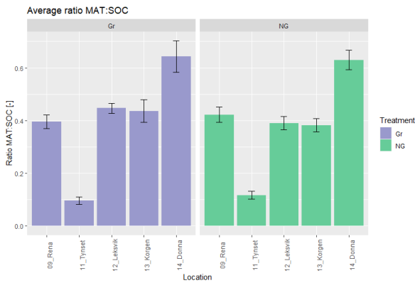
Appendix 13.1: Ratio of mean annual temperature (MAT) and average SOC stock [kgC/m2] by treatment and location. For treatment grazed (Gr) blue bars and non-grazed (NG) green bars. The locations are given on the x-axis.
