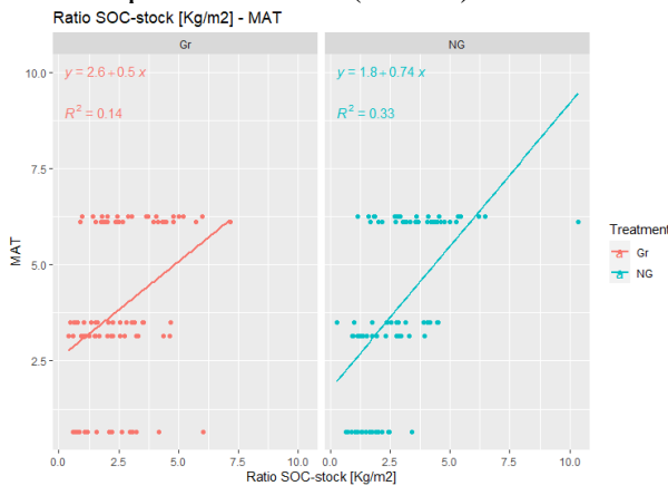
Appendix 13.5: linear regression between the MAT and average SOC stock [kgC/m 2 ] for all locations divided by treatment. The frame on the top side filters the locations, the frame on the top the treatment (Gr/NG).
