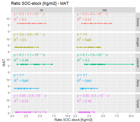
Appendix 13.3: linear regression between the MAT and average SOC stock [kgC/m 2 ] divided by treatment and location. The frame on the right side filters the locations, the frame on the top the treatment (Gr/NG).
