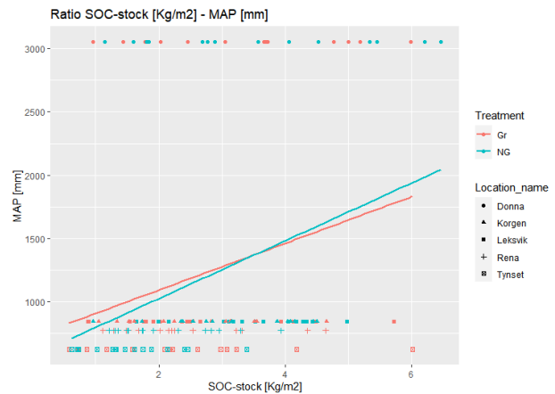
Figure 47: Linear relationship between the MAP [mm] and average SOC stock [kgC/m2] divided by treatment. The red line represents the grazed (Gr) sites and the blue the non-grazed (NG) sites. The symbols represent the locations.
