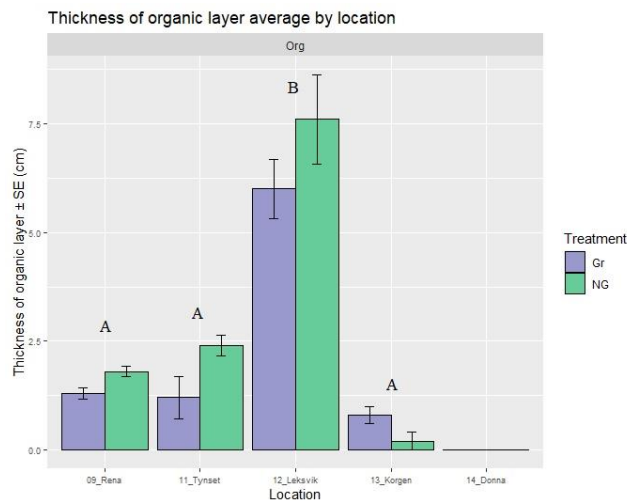
Figure 27: Average thickness of the organic layer [cm] ± standard error (SE) by treatment and location. The bars illustrate the thickness of the organic layer sorted by sites, grazed (blue) and non-grazed (green). The results are averaged by plots ( n=5 ), no organic layer was counted as a result. Dønna lacked organic layer. Capital letter indicates the difference between location (A, B). Groups with distinct letters are significantly different.
