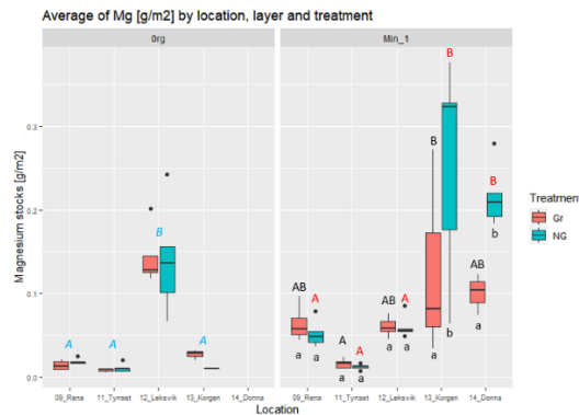
Figure 40: Average Mg-stocks of layer by treatment and location. The locations are grouped, the name is found on the x axis. The layers are grouped under frame found on top, respectively organic layer and min_1 (0-10 cm) The colour on boxes determine the treatment, grazed (red) and non-grazed (blue). Number of samples in each category displayed in the figure, see appendix 1.6. Notice that location Dønna do not contain a organic layer, and that Korgen, non-grazed site only contain one sample. The boxplots display the maximum and minimum by fully drawn line ad outliers is shown with a dot. Horizontal line inside the boxes represents the median of the category. In addition, lower case letters by the average value represents a significant difference between treatments (Gr/NG) within each location and the letter the difference between category (a, b, ab, c). Uppercase italic blue letters indicate a significant difference between locations ( A, B, AB ). Uppercase letters in black indicates differences between locations of the grazed outfields ( A, B, C, AB, BC ), and uppercase red letters indicate differences between locations for the non-grazed outfields ( A, B, C, AB, BC ). Different letters indicate differences at a level of significance p<0.05 .
