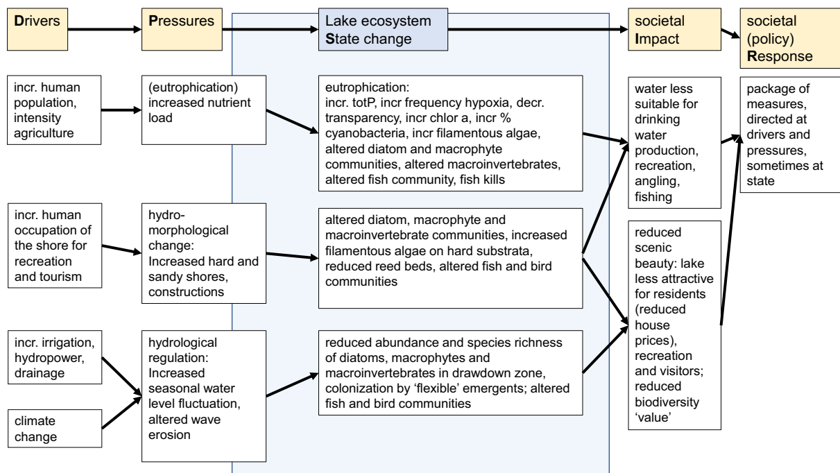
Fig. 1. Generalized a priori DPSIR framework combining three environmental pressures on Western Balkan lakes. A policy response can feed back to any of the other four elements.
