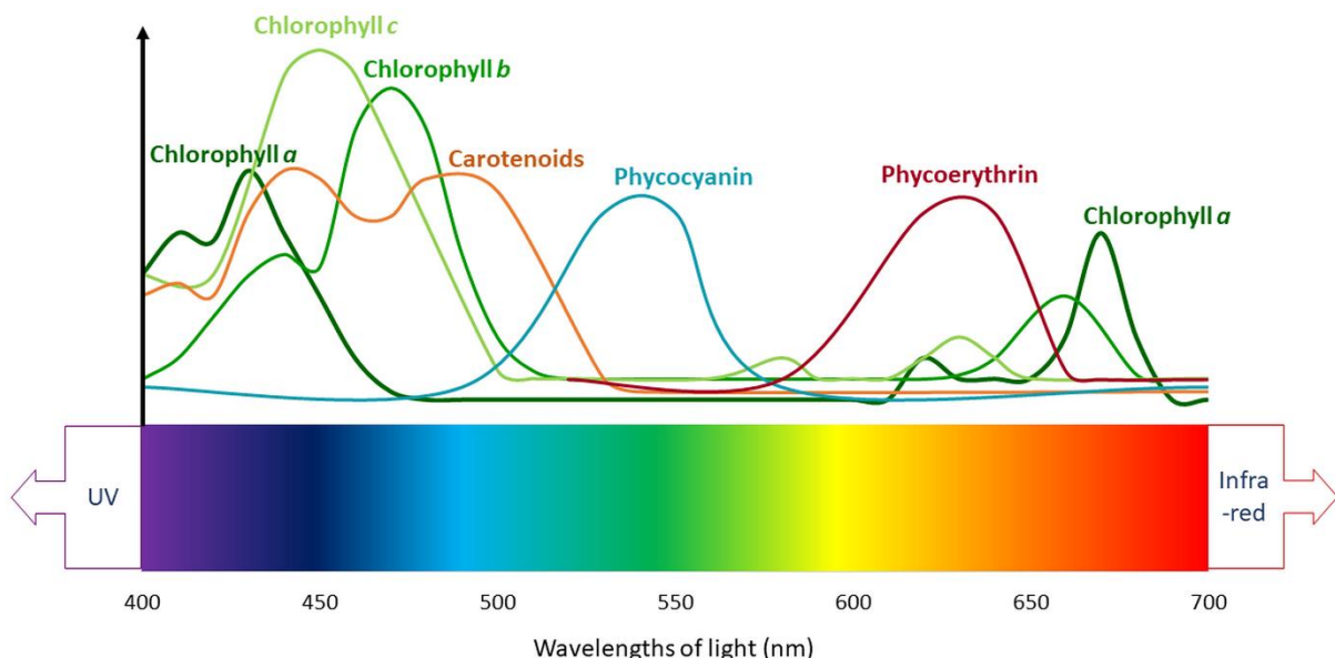
Figure 4. Absorption range of different algae pigments, including chlorophyll a , b , c , carotenoids and phycobilipigments (Roy et al. 2011), in the photosynthetic active radiation (PAR) spectrum of visible light.
