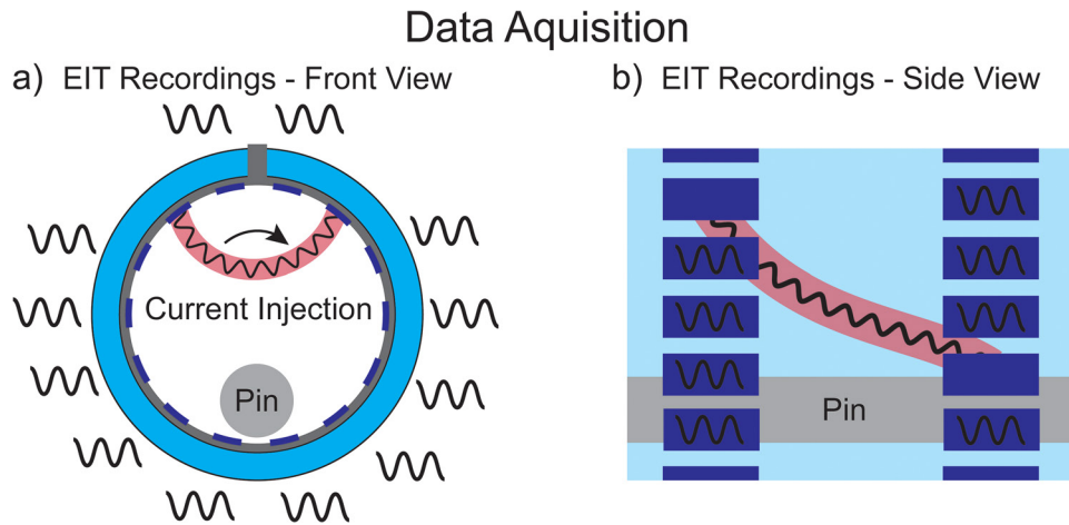
Figure 2. Schematic of a single recording of EIT data from an injection pair in both (a) front and (b) side view. The injection pair was then switched between the other electrodes to gather a full data set.
