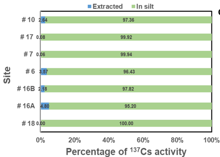
Figure 14: Proportion of ^{137}\text{Cs} leached in (A) total samples before size-segregation, (B) sand fraction, (C) silt fraction, and (D) clay fraction. Site 6, 7, 10, 16A and 17 are soils while 16B and 18 are sediments
