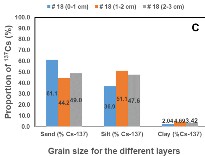
Figure 13. Proportion of ^{137}\text{Cs} contained in the different grain sizes at different levels of soils (A) and sediments (Band C)
