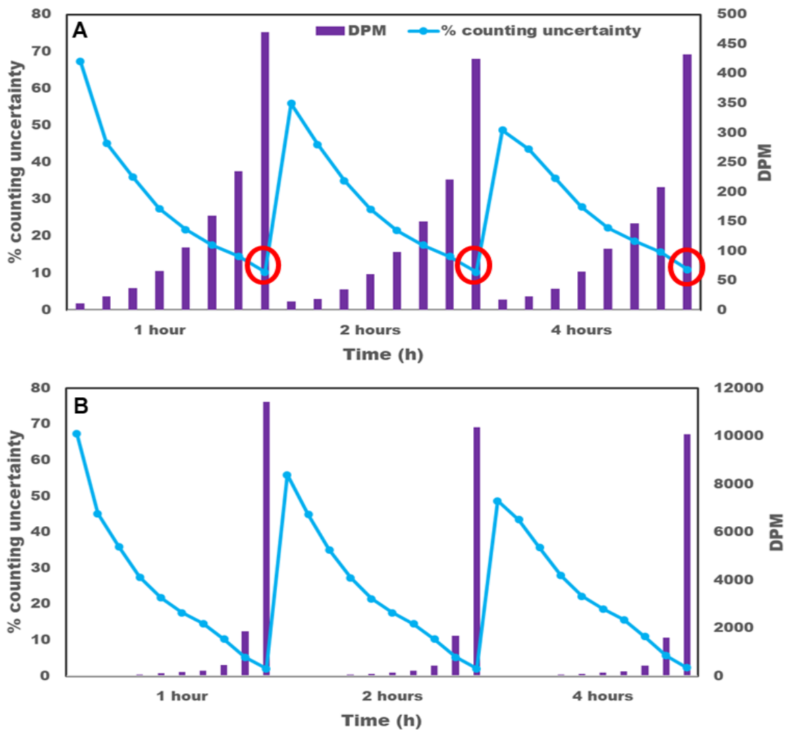
Figure 9: Effect of counting time on counting uncertainty: (a) activities < 500DPM (b) > 1000DPM
