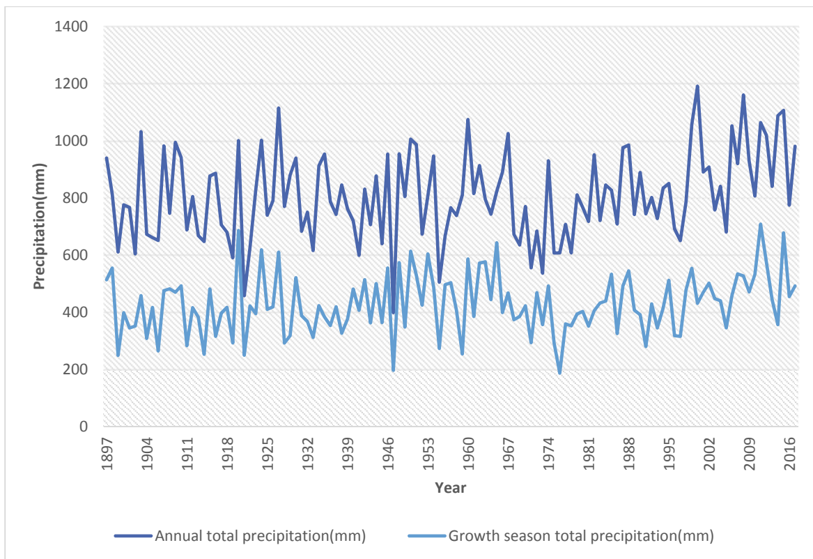
Figure 3.12: Annual total precipitation(mm) and growth season(April-September) total precipitation(mm). Figure is produced based on data provided by weather station BIOKLIM.
