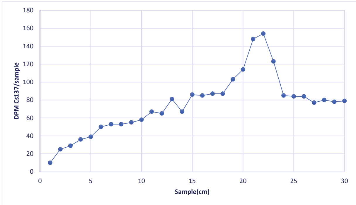
Figure 3.2: Distribution of Cs 137 down to a depth of 30 cm in the sediment core obtained from lake Grepperødfjorden. Each sample represents 1 cm.
