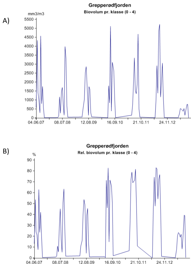
Figure 2.8: A) Biovolume distribution of Raphidophyceae in lake Grepperødfjorden during the growth seasons of 2007-2013. B) Percentage contributions of Raphidophyceae to total biomass during the growth seasons of 2007-2013 (Aquamonitor, n.d.b)
