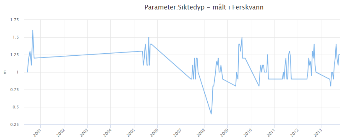
Figure 8D: Development of secchi depth in lake Grepperødfjorden during the monitored period of 2000, 2005 and 2007-2013. Source: vanmiljo.miljodirektoratet.no . Retrieved 24.4.2018.
