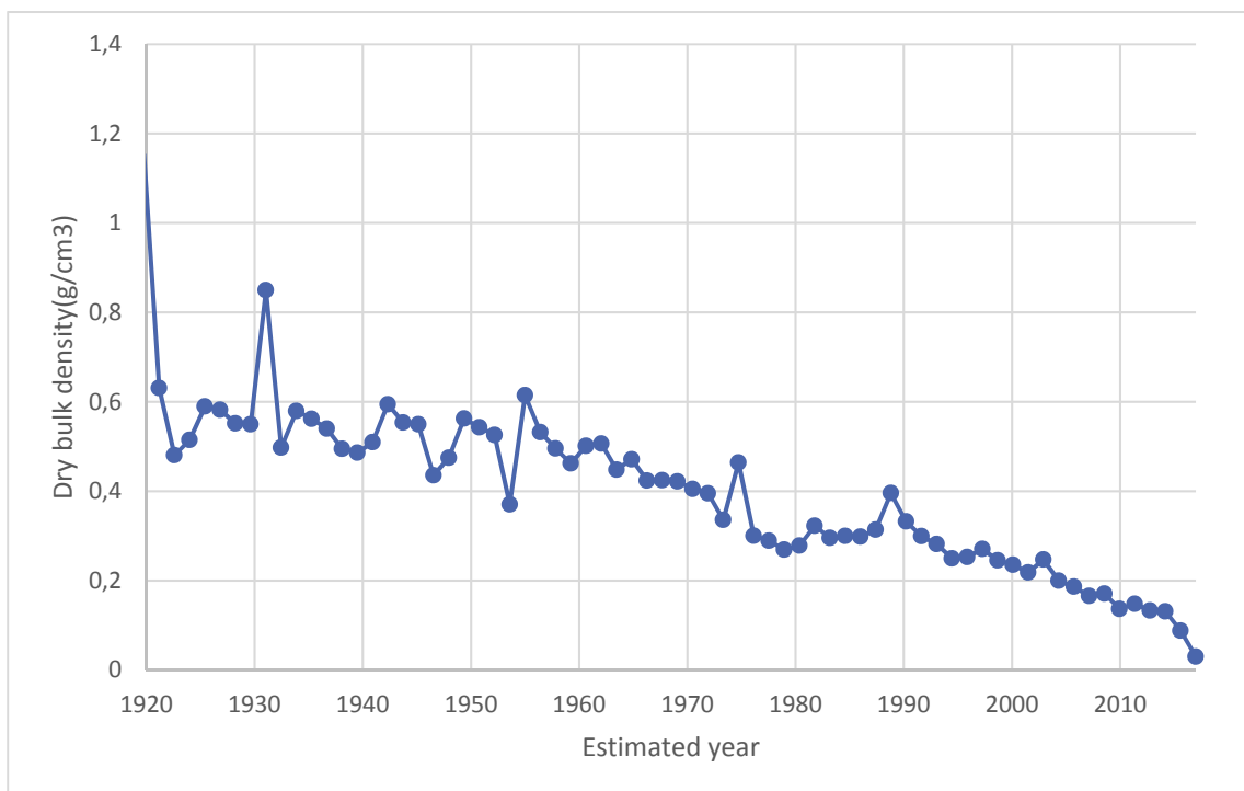
Figure 3.10: Dry sediment bulk density ( \text{g/cm}^3 ) distribution throughout the estimated time span in the sediment core obtained from lake Grepperødfjorden. Bulk density values have in general declined as time has progressed, suggesting increasing levels of organic matter in the sediments.
