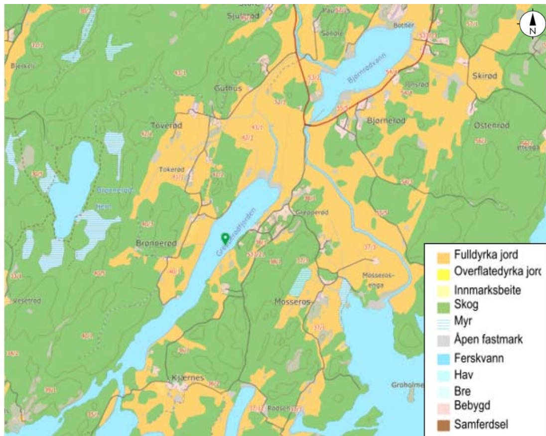
Figure 2.5: Land use map (1:40 000) of lake Grepperødfjorden drainage basin. Legend is given in Norwegian. Drainage basin area is heavily influenced by agricultural activity( orange color). Agriculture is concentrated in the northern and north-western end of the lake. Human settlement is mainly found at Grepperød in north-east and at Kjærnes in south-east. Map is modified from NIBIO(n.d.b)
