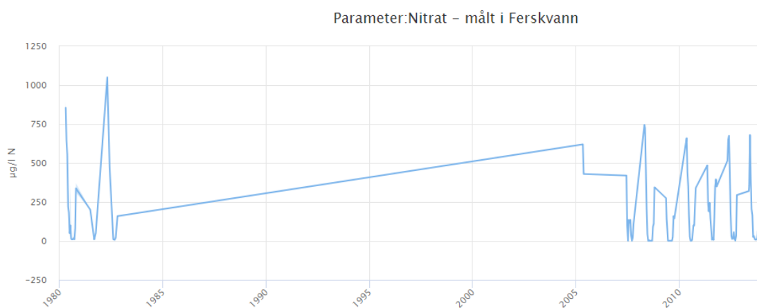
Figure 8C: Development of NO 3 -N in the water phase of lake Grepperødfjorden during the monitored period of 1980-1982, 2005 and 2007-2013. Source: vanmiljo.miljodirektoratet.no . Retrieved 24.4.2018.
