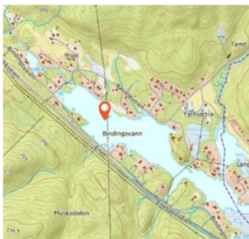
Figure 2.9: Sediment core sampling location for lake Bindingsvann (kartverket.no)
