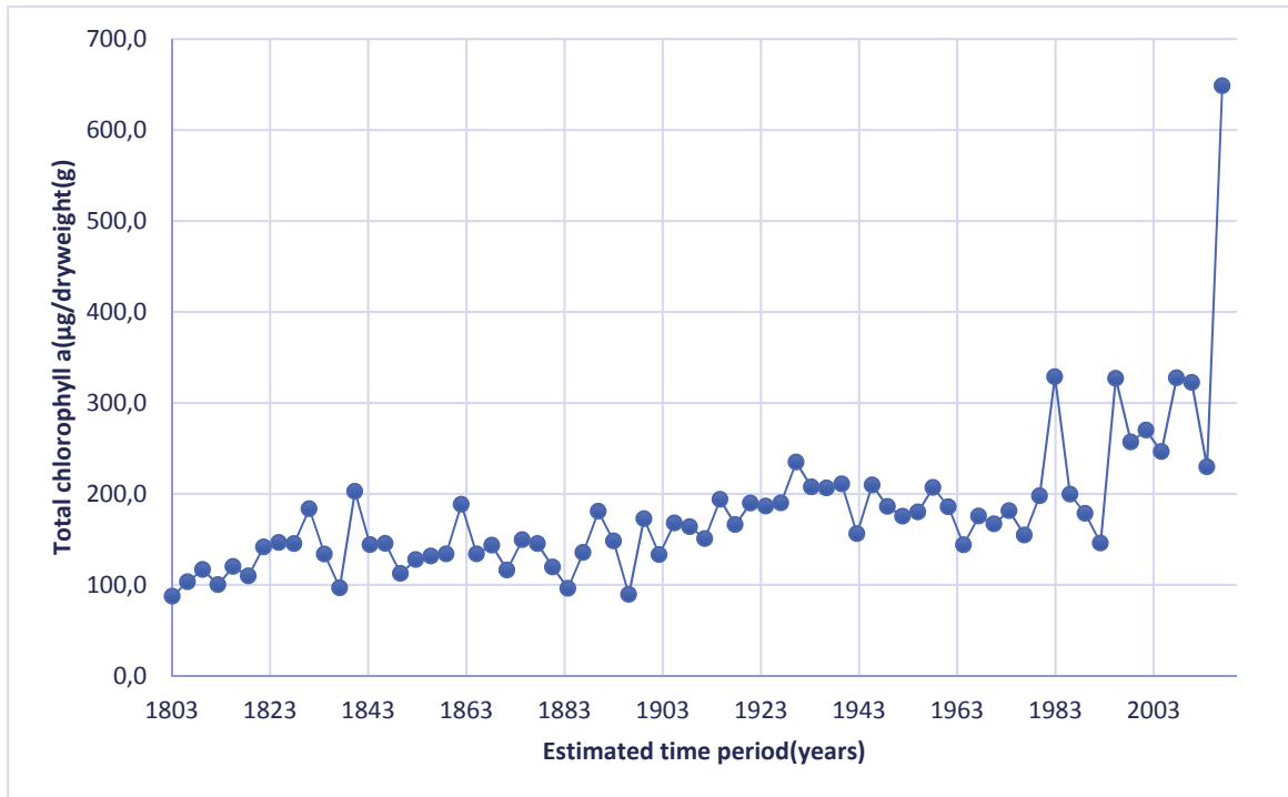
Figure 3.3: Estimated sediment core distribution of total chlorophyll a (the sum of chlorophyll a and its breakdown product pheophytin a) for lake Bindingsvann.
