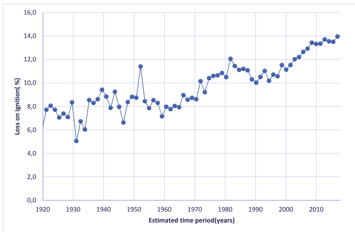
Figure 3.8: Loss on ignition (%) for lake Grepperødfjorden during the estimated period of 1920-2017.
