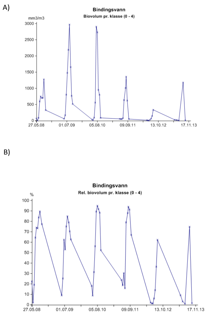
Figure 2.4: A) Biovolume ( \text{mm}^3/\text{m}^3 ) of Raphidophyceae during the growth seasons of 2008-2013. Gonyostomum is the most common representative of this class. B) Percentage contribution of Raphidophyceae to total biovolume in lake Bindingsvann during the growth seasons of 2008-2013 (Aquamonitor, n.d.a)
