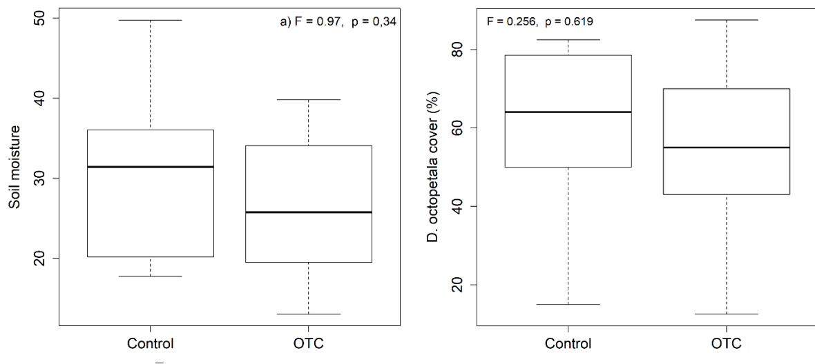
Figure 5a: Differences in soil moisture between OTCs and control plots. Figure 5b: Cover of Dryas Octopetala in OTCs and control plots. F- and P-values are obtained from ANOVA-analysis. The boxplots show the median and the interquartile range.
