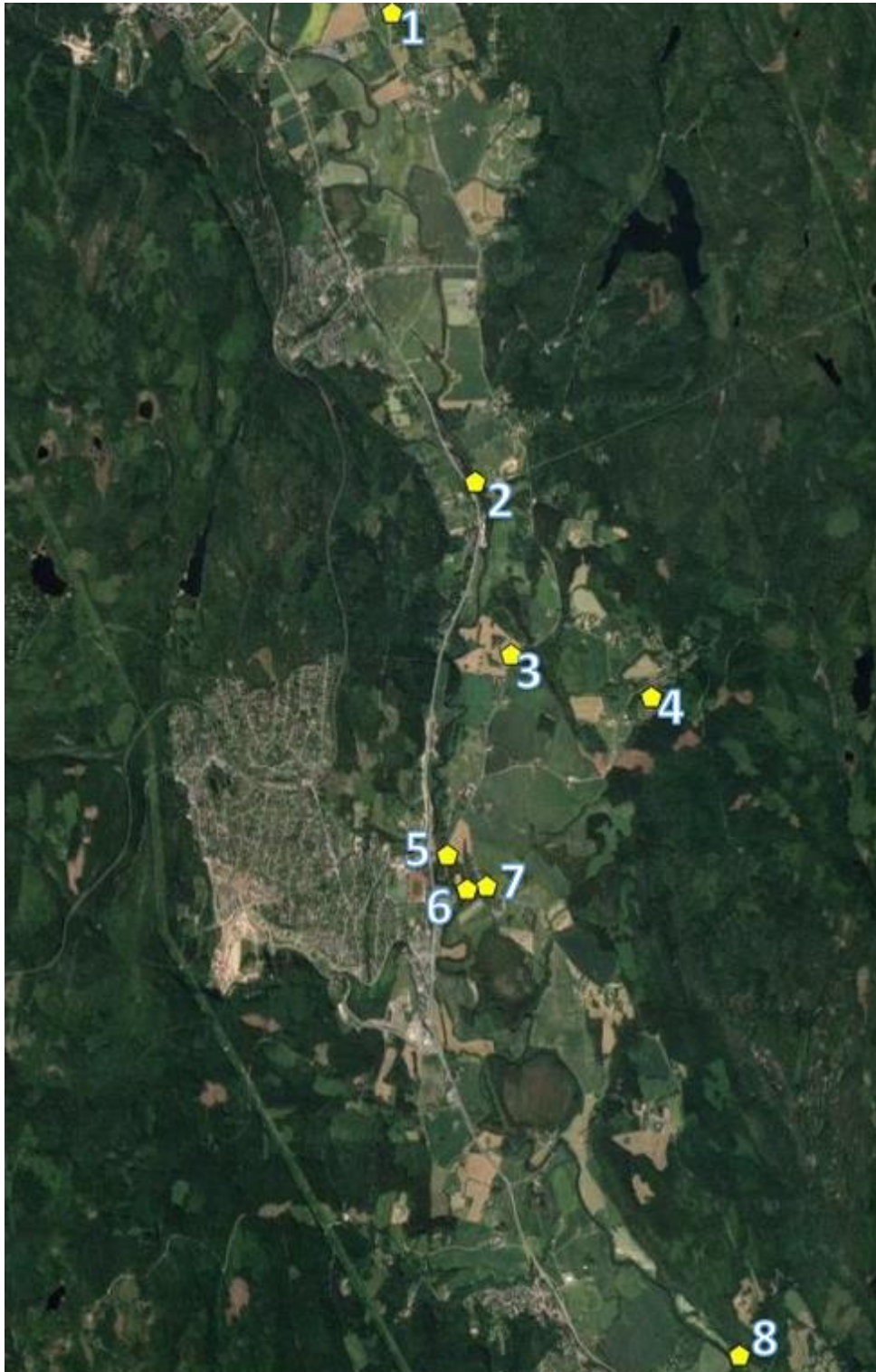
Figure 7: 1:147585. Map of all maternity colonies located (yellow pentagrams). Colonies numbered for ease of recognition in no particular order. Colony number one was not found as part of this study, but was known from van der Kooij (2012).
