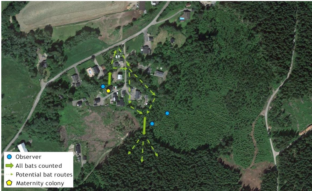
Figure 15: Scale:1:4162. Shows the perceived route that the bats ( M. brandtii , female) of the Ask colony (presumed maternity colony) used. This is based on visual observations, counting, bat detector usage and signals from the tagged bats. The observer markers are used to highlight important positions that were used to either determine or exclude possible bat routes. The potential bat routes are suggestions based on what we see as the most likely path the bats took. They were not necessarily there on the same day and not necessarily the same observer. Tags lasted from 12.06 to 20.06 for #049 and 22.06 for #203.
