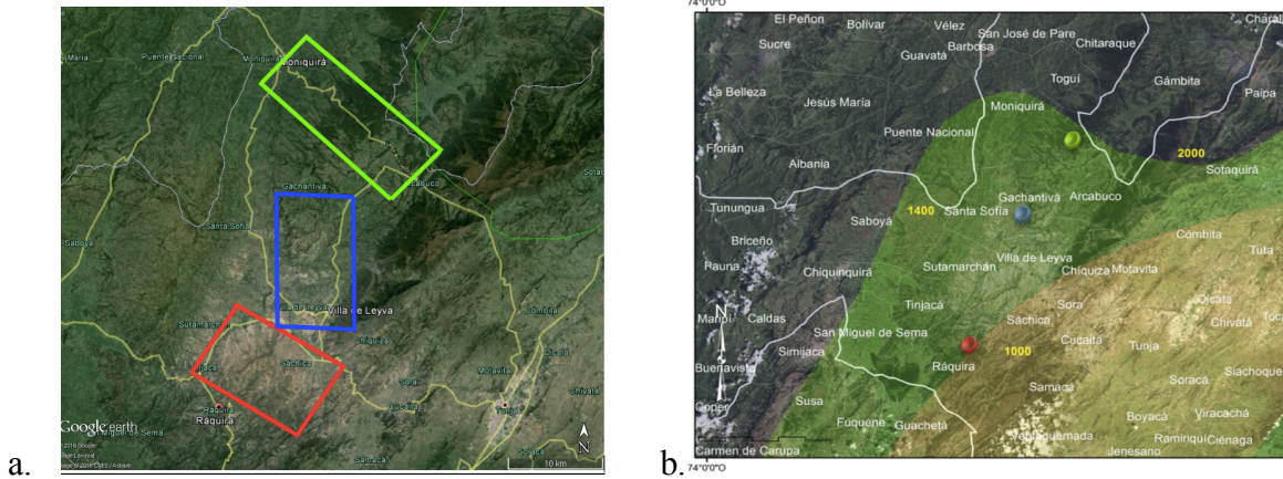
Figure 3: (a) Three polygons showing the study area in the Ricaurte Province based on a humidity gradient: High humidity - Moniquira/Arcabuco in green; Moderate humidity - Gachantiva in blue; and low humidity - Raquira in red. (b) The tree location sites (dots) and the three humidity belts present in the Province of Ricaurte; lemon-colour area represents lower humidity; green area represents moderate humidity and dark green represents high humidity. Yellow numbers show Annual mean precipitation (mm). Source: created on GoogleEarth, 2016.
