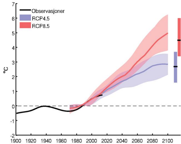
Figure 3: Deviations for annual temperature in °C, for Norway relative to reference period 1971-2000. The black line illustrates observational values, the blue is median simulation values for RCP4.5, and the red RCP8.5. The faded colour indicates the spread between high and low simulation values. All curves are smoothed. (Hanssen-Bauer et al. 2015)
