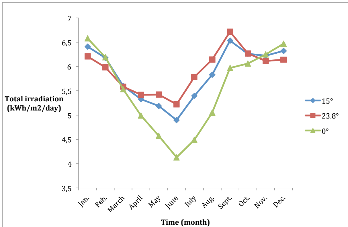
Figure 5-4: Total daily irradiation ( \text{kWh/m}^2/\text{day} ) at horizontal, 15^\circ tilted and 23.8^\circ degree tilted surface in Polokwane (Atmospheric Science Data Center)
