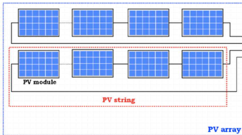
Figure 3-2: PV array arrangement (Manna, 2014)
