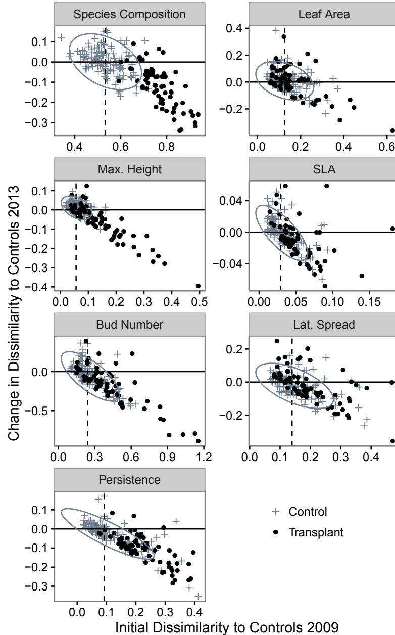
FIG. 3. Changes in dissimilarity of turfs transplanted to warmer climates and target site controls from 2009 to 2013. The x -axis shows Bray–Curtis dissimilarity between turfs and the centroids of their control turfs in 2009; the y -axis shows how that dissimilarity changed by 2013. Each symbol represents a turf community. Grey crosses represent control turfs; black circles represent transplanted turfs. Dissimilarity was calculated using Bray–Curtis distance for species composition (top left panel) or Euclidian distance of community weighted means (all remaining panels). Symbols below zero on the y -axis reflect turf communities that converged compositionally towards target controls, whereas communities above zero on the y -axis diverged compositionally. Dashed vertical lines are placed at 50% of mean dissimilarity among controls as an approximation of natural community stochasticity. Grey ellipses represent 95% confidence intervals of the centroids of control turf dissimilarities.
