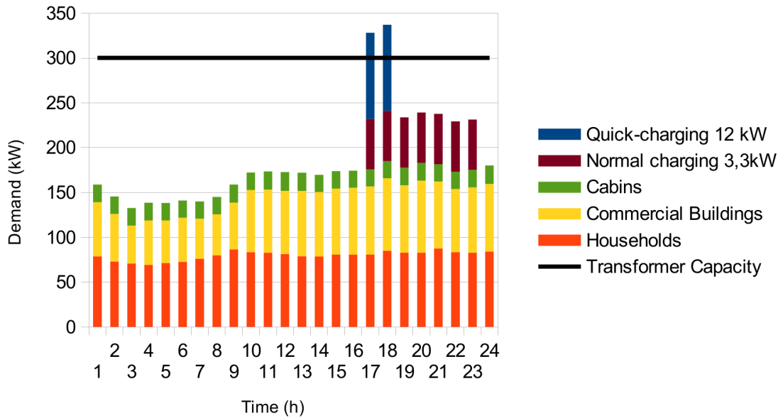
FIGURE 3.7: Load Profiles of a 315kVA distribution transformer serving 25 homes, 25 cabin, 11 commercial buildings and 25 EVs charging were 13 are charged with 3,3kW and 12 with 12 kW (quick charge) in the peak evening hours on the 23/01/2013.
