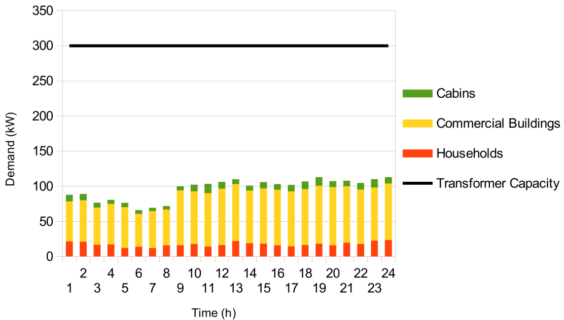
FIGURE 3.4: Load Profiles of a 315kVA distribution transformer serving 25 homes, 25 cabin, 11 commercial buildings on the 22/07/2013.
