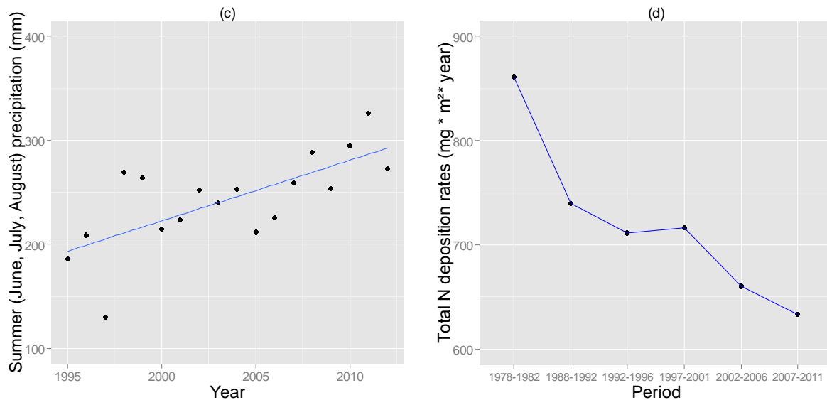
Figure 2 Scatter plots showing temporal variation of annual and summer (June, July and August) temperature (a) and precipitation (b) in the period 1975–2012, in addition to total summer precipitation in the period between 1995 and 2012 (c) (linear regression, total summer precipitation = -11446 + 5.8\text{Year} , p < .01 , n = 18 ) and 5-year interval estimates of atmospheric N deposition in the region of the study area (d).
