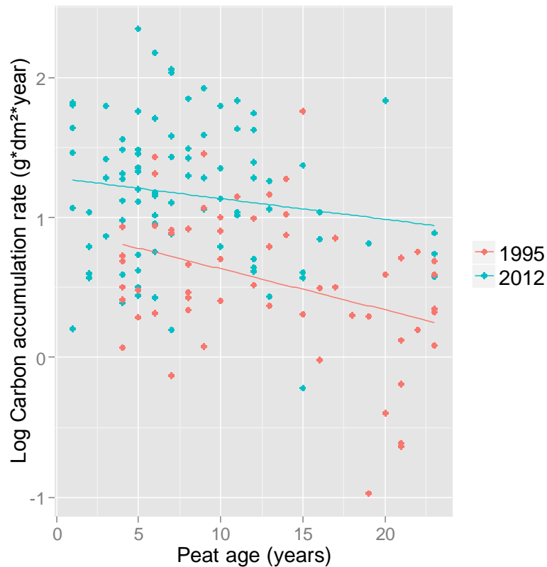
Figure 6 Relationship between (log) carbon accumulation rate and peat age for the two sampling years.
