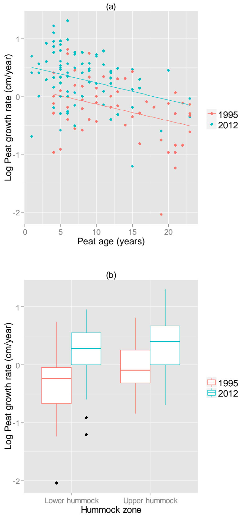
Figure 4 Relationship between (log) peat growth and age (a) and (log) peat growth and affiliation to hummock zone (b) for the two sampling years.
