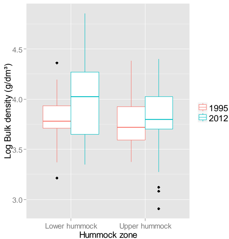
Figure 5 Relationship between (log) bulk density and hummock zone for the two sampling years showing an overall increase in bulk density in 2012 samples.
