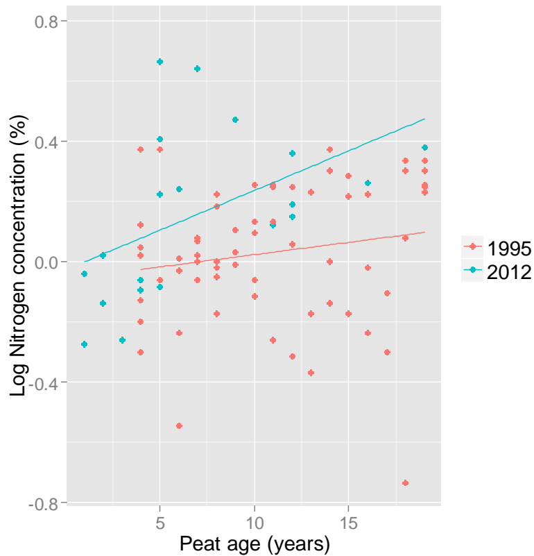
Figure 7 Relationship between (log) N concentration and peat age for the two sampling years.
