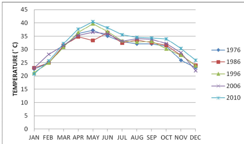
Figure 7. Monthly maximum temperatures of Rani Jaruwa Nursery for the years 1976, 1986, 1996, 2006 and 2010
