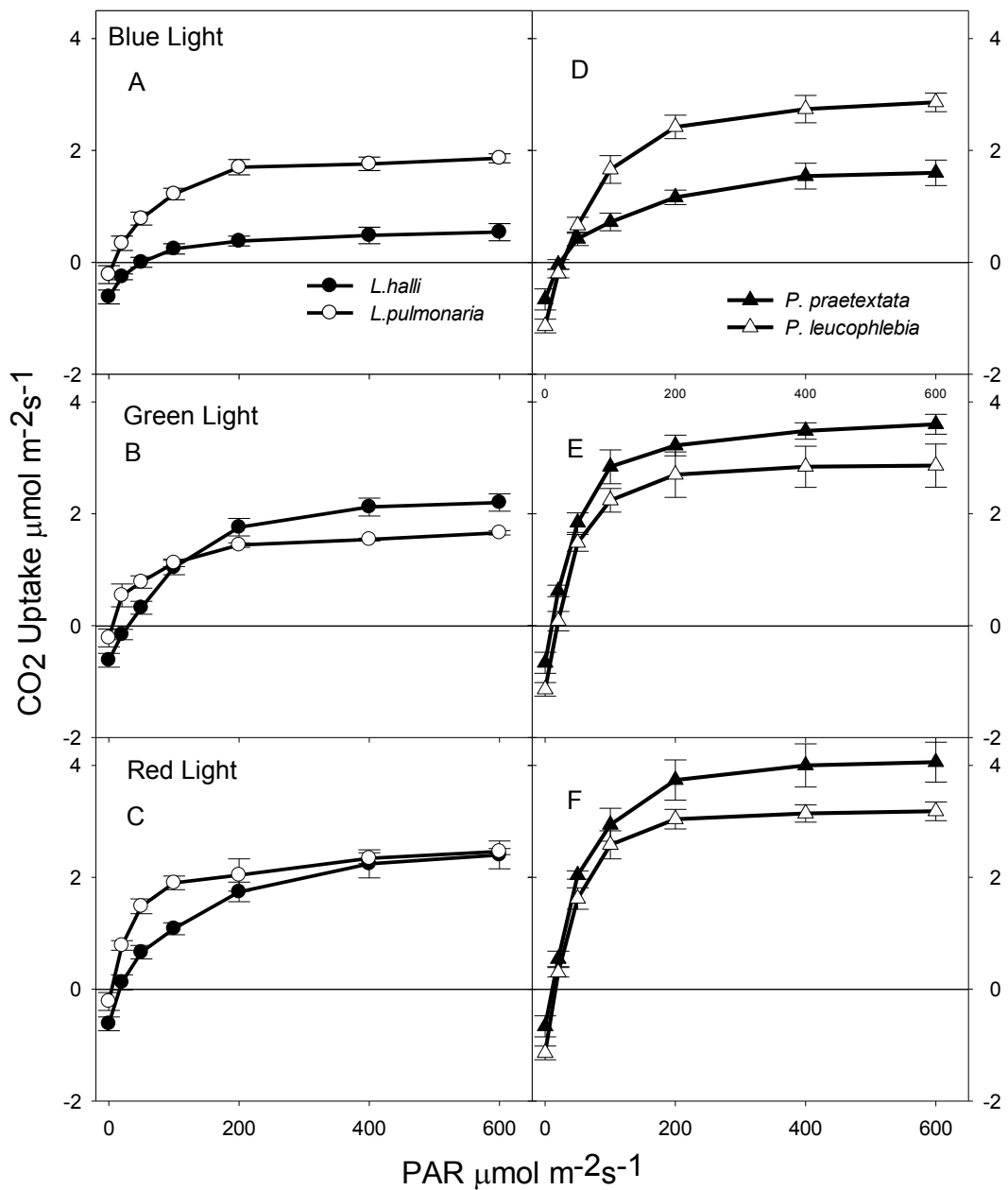
Figure 11 Light response curves for CO 2 uptake for Lobaria pulmonaria and L. hallii (A, B and C) and for Peltigera leucophlebia and P. praetextata (D, E and F) in blue (A and D), green (B and E) red (C and F) light. Before measurement all thalli were acclimated in hydrated condition for 24h at 30 \mu\text{mol photons m}^{-2} \text{s}^{-1} . Each curve is the mean of light response curves for 10 thalli. The error bars show SE.
