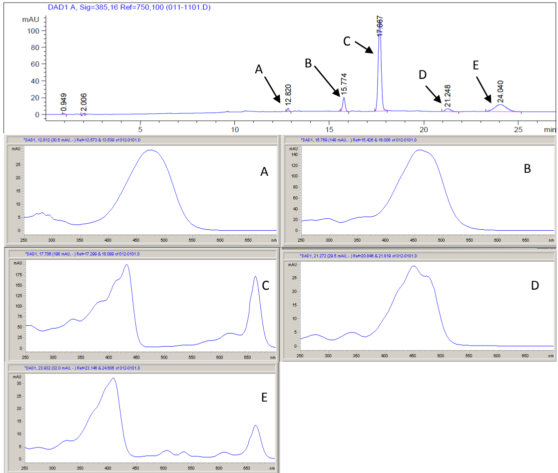
Figure 15 HPLC chromatogram of P. praetextata with spectra for the individual peaks record with the HPLC photodiodearray detector. A, B and D are carotenoids. C and E are chlorophyll a.
