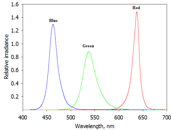
Figure 5 SL3500 LED light source
