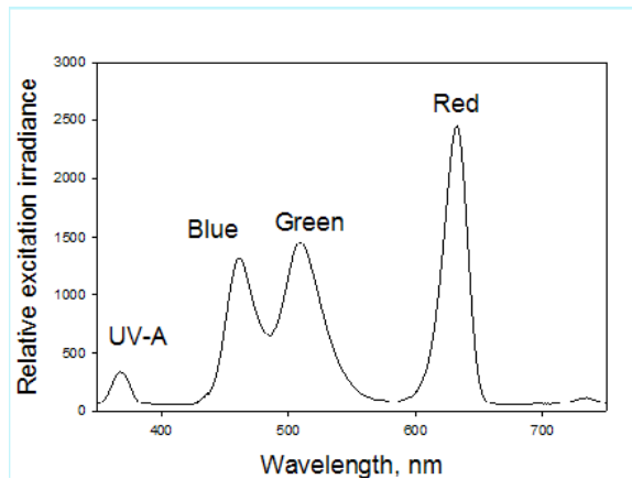
Figure 6 Excitation wavelengths of the “Multiplex” instrument
