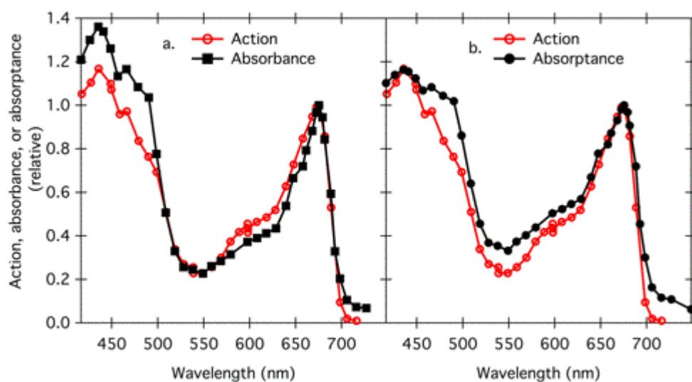
Figure 1 Action spectrum of photosynthesis in green algae Ulva plotted with (a) thallus absorbance and (b) thallus absorptance (Haxo and Blinks, 1950).
