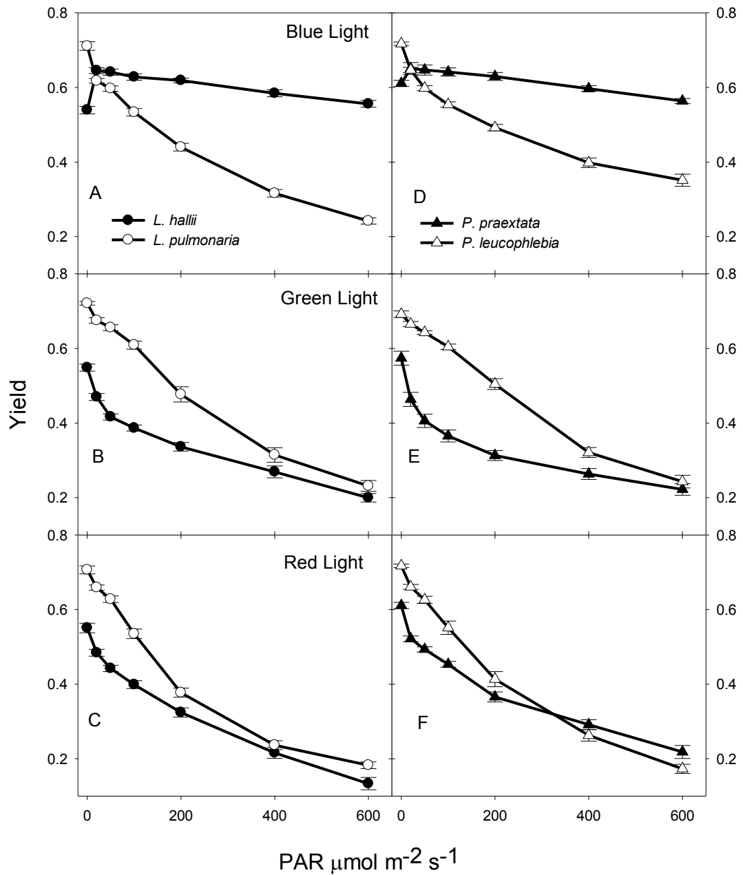
Figure 9 Light response curves of yield value for L. pulmonaria and L. hallii (A, B and C) and for P. leucophlebia and P. praetextata (D, E and F) in blue (A and D), green (B and E) red (C and F) light. Each curve is the mean of light response curves for 10 thalli and the error bars show SE.
