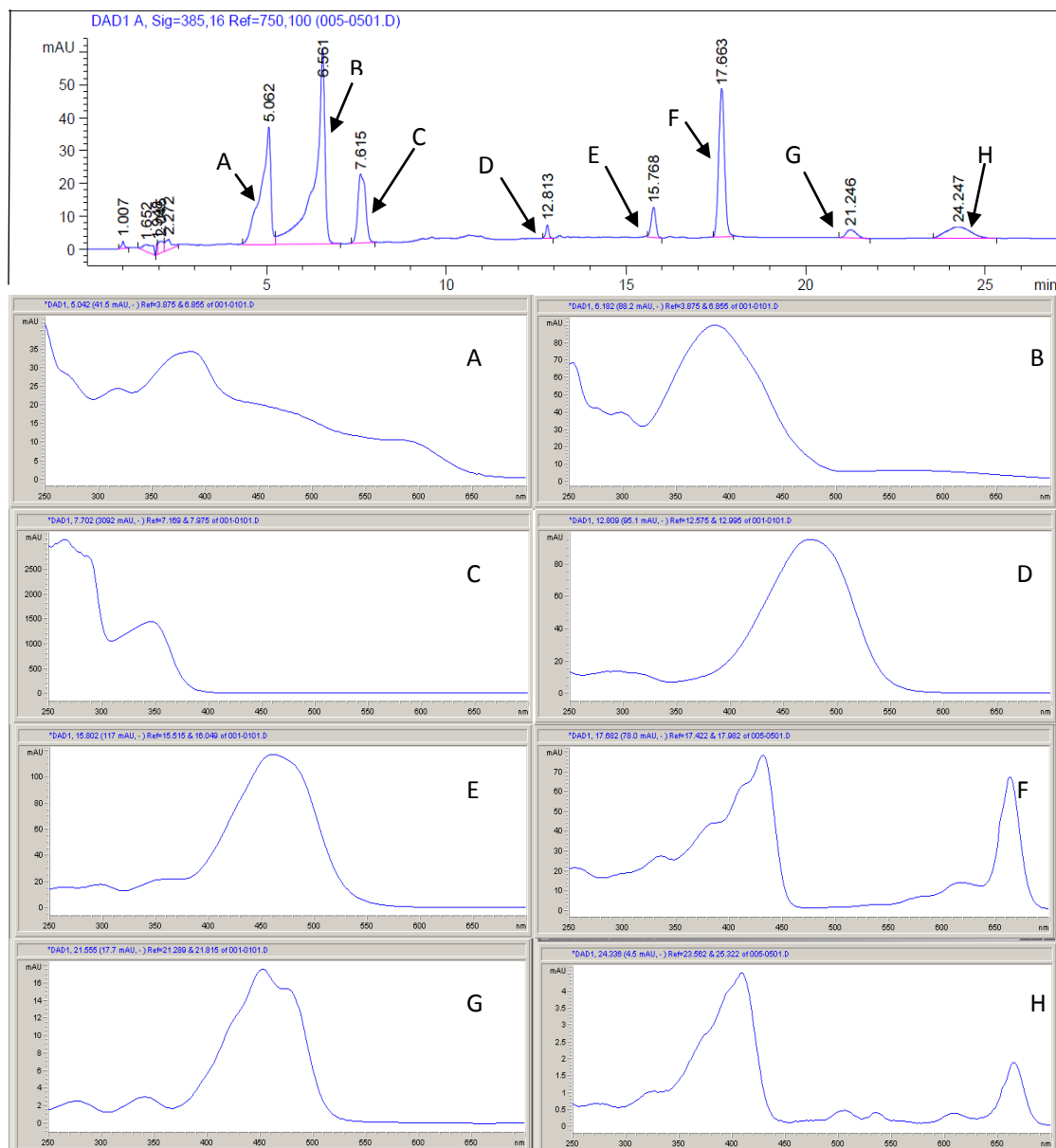
Figure 14 HPLC chromatogram of L. hallii with spectra for the individual peaks recorded with the HPLC photodiodearray detector. A is red scytonemin (Mueller et al., 2005). B is scytonemin. C is some unknown substance. D, E and G are carotenoids. F and H are Chlorophyll a.
