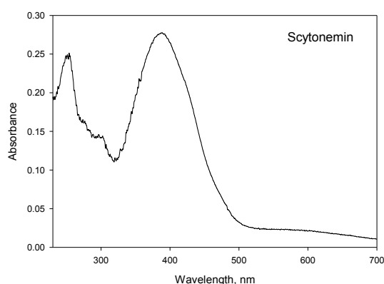
Figure 8 The spectra of scytonemin standard which was measured by UVPC. the standard scytonemin was extracted by HPLC from lichen species L. hallii .
