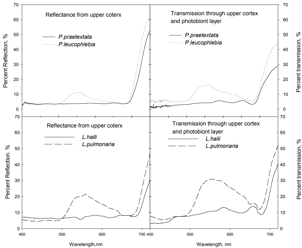
Figure 13 Reflectance from upper cortex and transmission through upper cortex and photobiont from thalli of L. hallii , L. pulmonaria , P. praetextata and P. leucoplaebia . Each curve is the average of five measurements.
