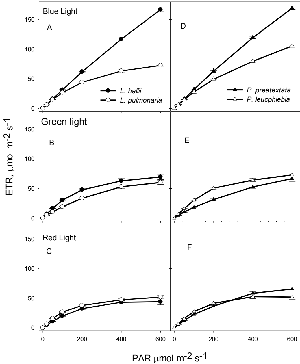
Figure 10 Light response curves of apparent ETR for Lobaria pulmonaria and L. hallii (A, B and C) and for Peltigera leucophlebia and P. praetextata (D, E and F) in blue (A and D), green (B and E) red (C and F) light. Each curve is the mean of light response curves for 10 thalli and the error bars show SE.
