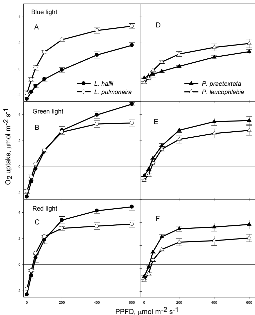
Figure 12 Light response curves for photosynthetic O 2 evolution for thalli genus Lobaria and Peltigera . Before measurement all thalli were acclimated in hydrated condition for 24h at 30 \mu\text{mol photons m}^{-2} \text{s}^{-1} . Each curve is the mean of light response curves for 10 thalli. The error bars show SE.
