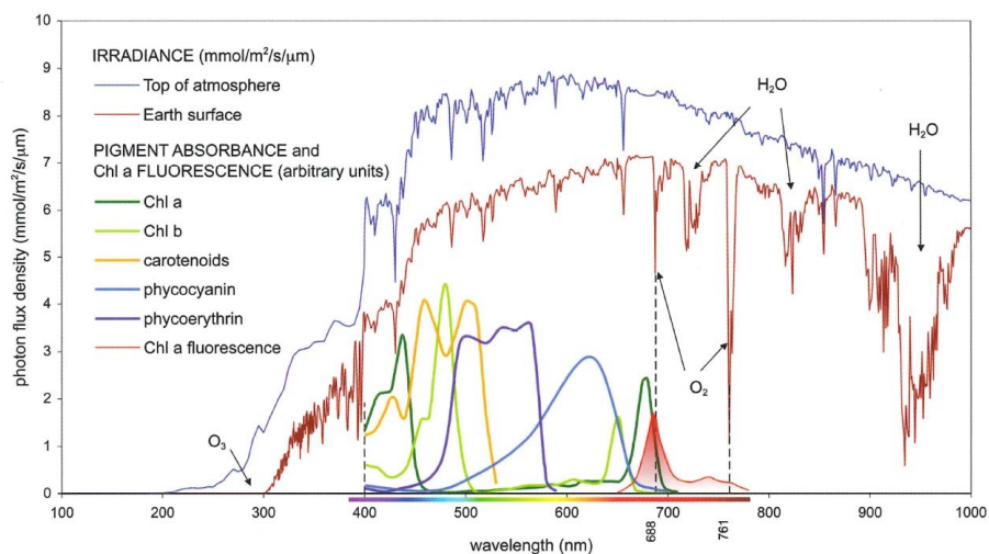
Figure 16. Irradiance and absorbance of various photosynthetic pigments. Cover page of (Papageorgiou and Govindjee, 2004)
