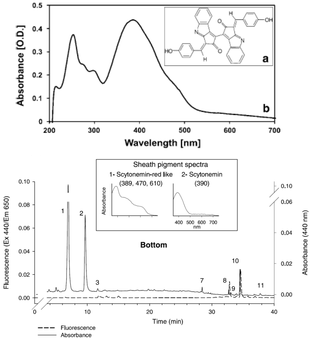
Figure 2 Upper panel: Structure of scytonemin (a) and its absorption spectrum showing a maximum at 386 nm (b) (Rastogi et al., 2010). Lower panel: HPLC chromatogram from a microbial mat sample from Markham Ice Shelf with spectrum of the scytonemin peak and the scytonemin-red like peak (Vincent et al. 2004).
